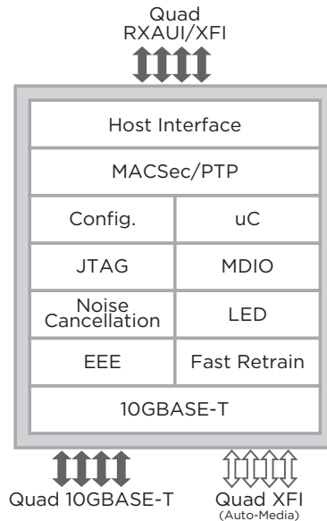
Fig 1. Marvell Alaska X 88X3240P
