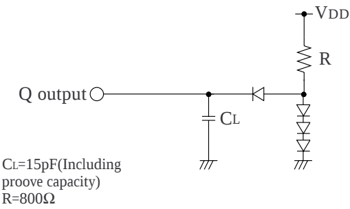
Load Circuit 2
