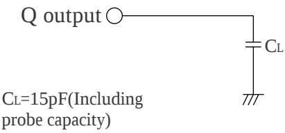
Load Circuit 1
