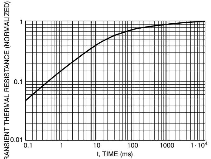
Figure 4. Thermal Response
