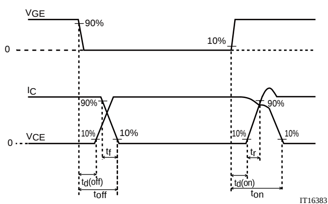
Fig.2 Timing Chart
