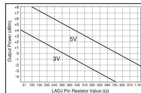
Figure 5: Output Power vs. LADJ Resistor
