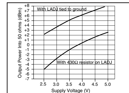
Figure 4: Output Power vs. Supply Voltage
