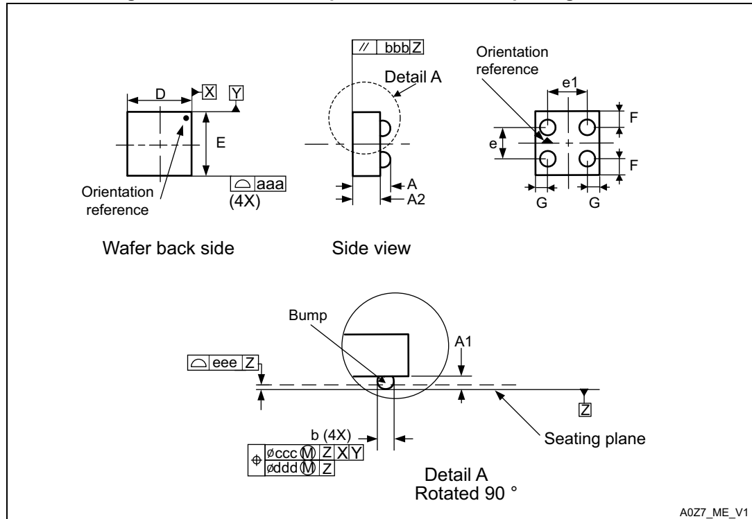
Figure 12. WLCSP 4-bump M24128S-FCU6T/T package outline
