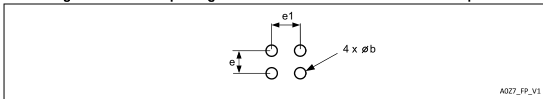
Figure 13. WLCSP package M24128S-FCU6T/T recommended footprint
