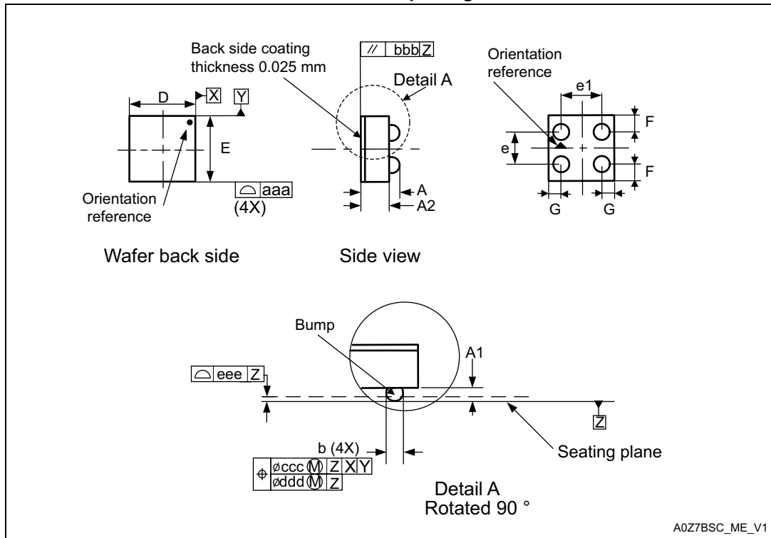
Figure 14. WLCSP 4-bump ultra-thin with Back Side Coating (BSC) M24128S-FCU6T/TF package outline
