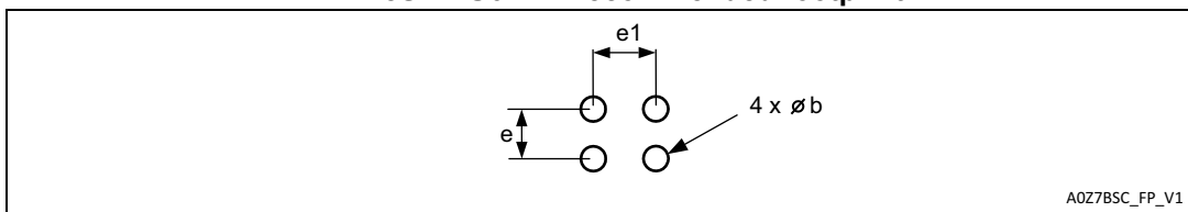
Figure 15. WLCSP package with Back Side Coating (BSC) M24128S-FCU6T/TF recommended footprint
