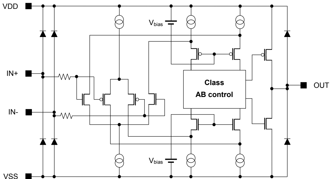
Figure 1. Simplified Schematic
