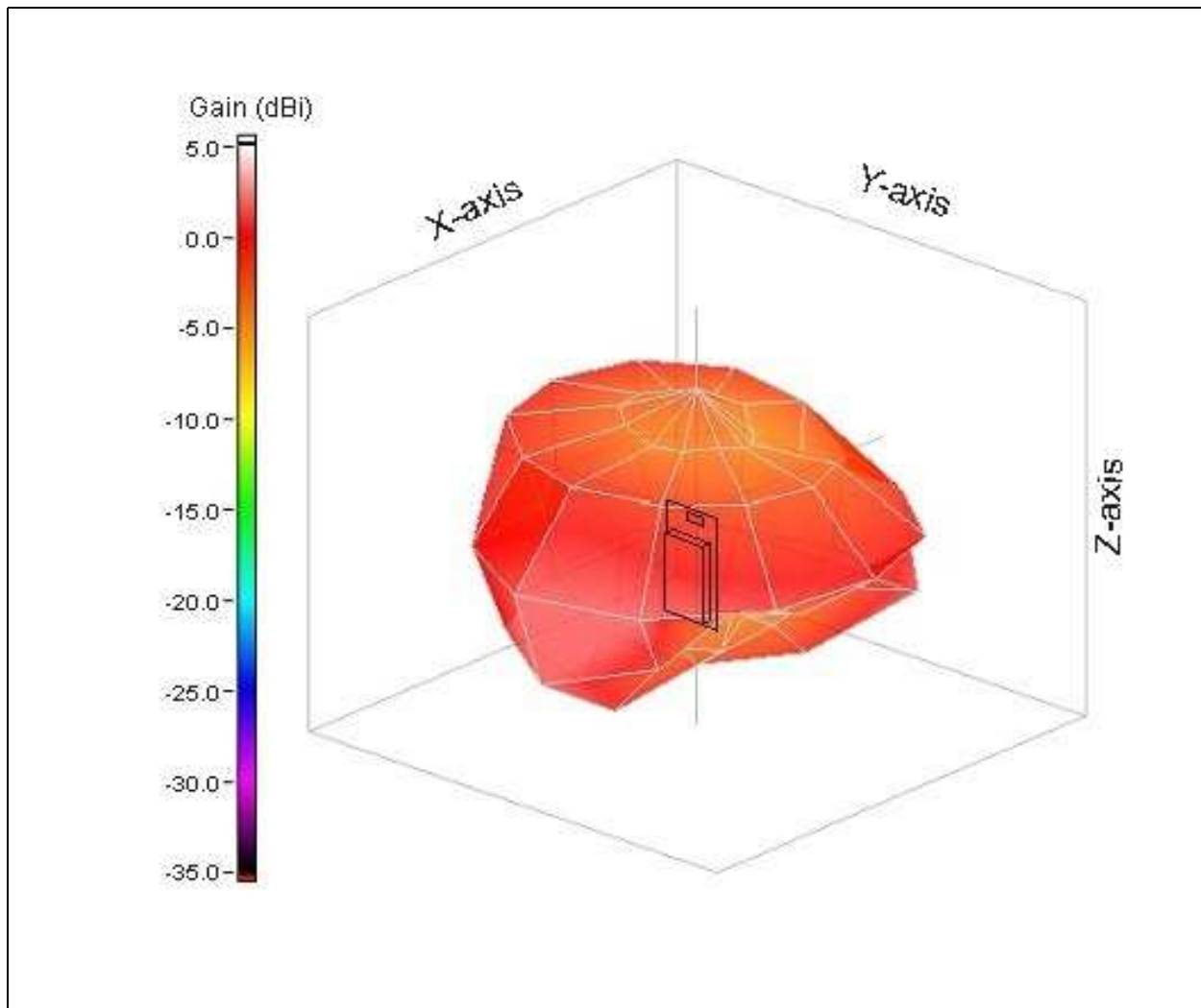
FIGURE 4-1: BM70BLES1FC2 ANTENNA RADIATION PATTERN
