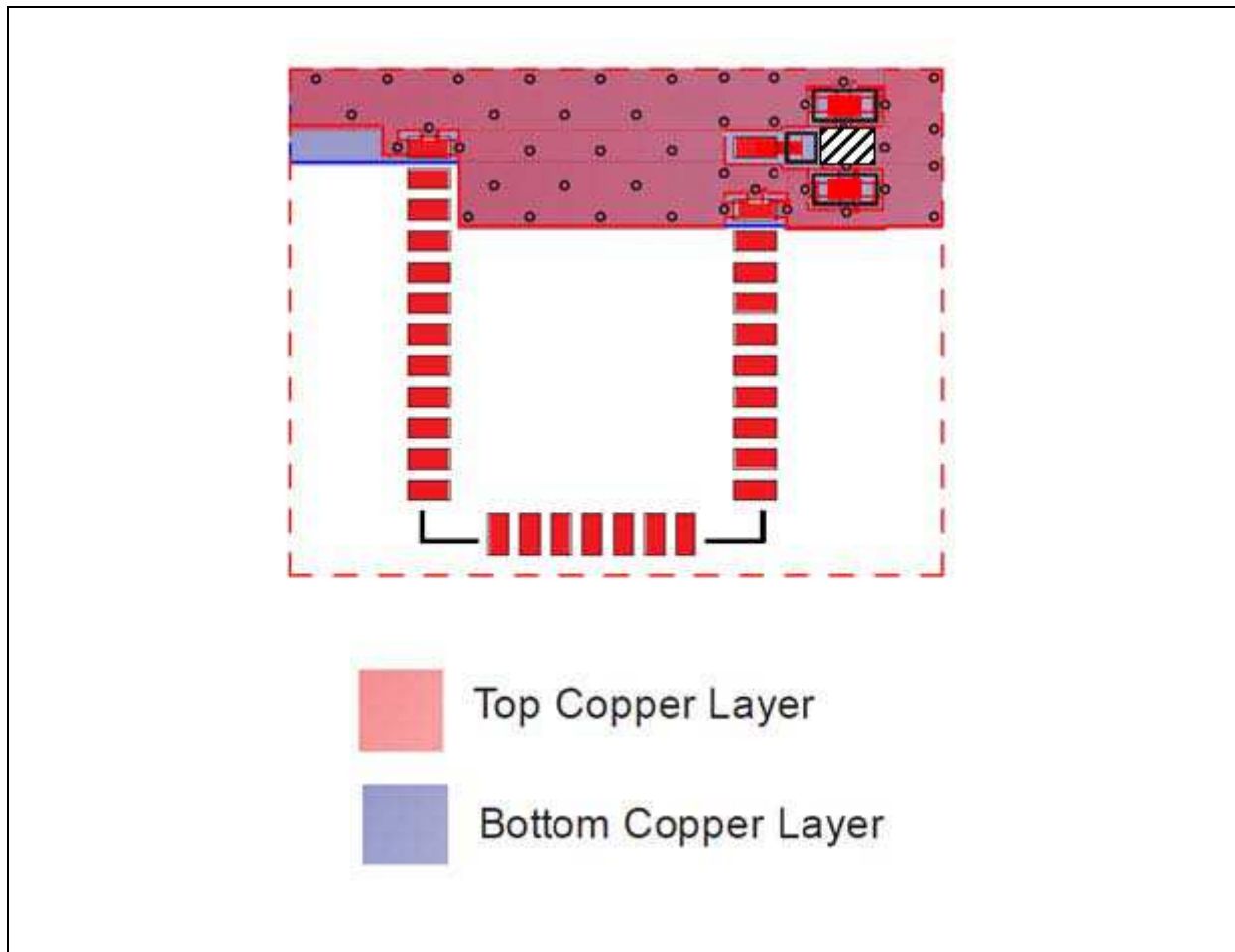
FIGURE 4-6: BM70BLE01FC2 HOST PCB MOUNTING SUGGESTIONS
