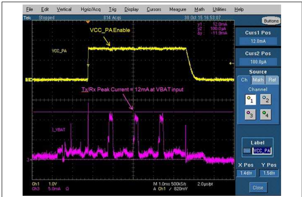
FIGURE 5-1: TX/RX PEAK CURRENT CONSUMPTION OF ADVERTISING EVENT IN BLEDK3 BEACON MODE
