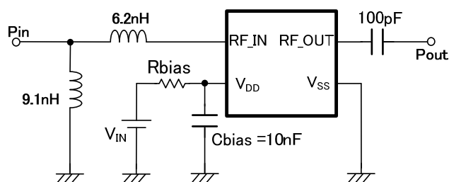
Figure 2: Self Bias
