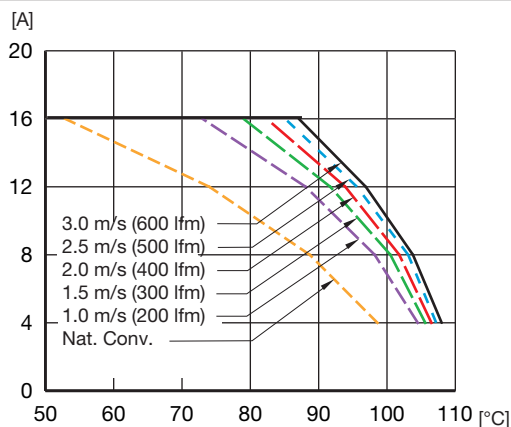
Available load current vs. ambient air temperature and airflow at V_{\text{in}} = 12\text{ V} . See conditions on page 30.
