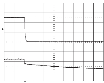
Turn-off at I_O = 16\text{ A} resistive load at T_{\text{ref}} = +25\text{ }^{\circ}\text{C} , V_{\text{in}} = 12\text{ V} . Turn-off enabled by disconnecting V_{\text{in}} . Top trace: output voltage (2 V/div.). Bottom trace: input voltage (10 V/div.). Time scale: 2 ms/div.
