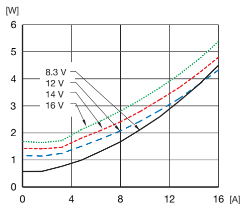
Dissipated power vs. load current and input voltage at T_{\text{ref}} = +25\text{ }^{\circ}\text{C}
