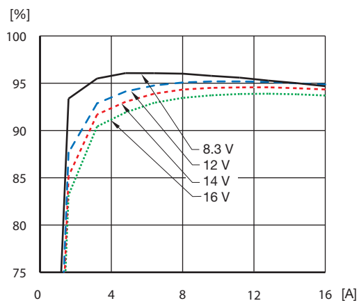
Efficiency vs. load current and input voltage at T_{\text{ref}} = +25\text{ }^{\circ}\text{C}
