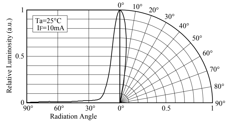
■ Directivity (NSPE500S)
