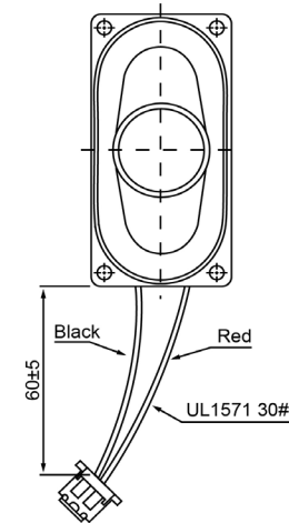
BOTTOM VIEW
