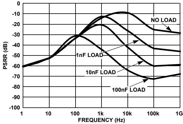
FIGURE 49. PSRR vs CAPACITIVE LOAD
