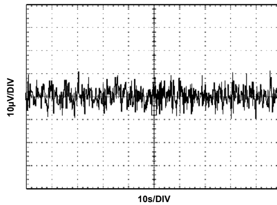
FIGURE 83. V_{OUT} NOISE
