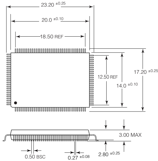
128 pin MQFP All dimensions in millimetres
