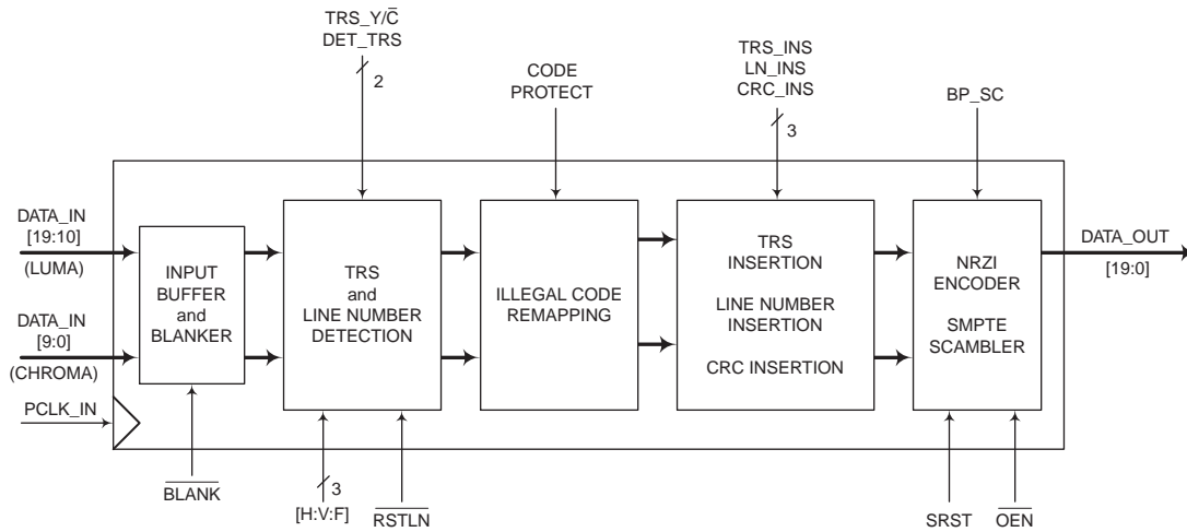
BLOCK DIAGRAM
