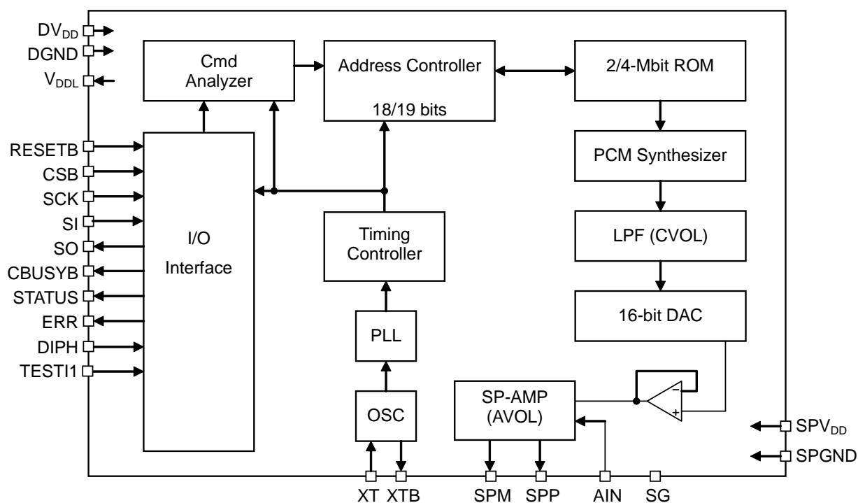
Block Diagram of ML2257X-xxx
