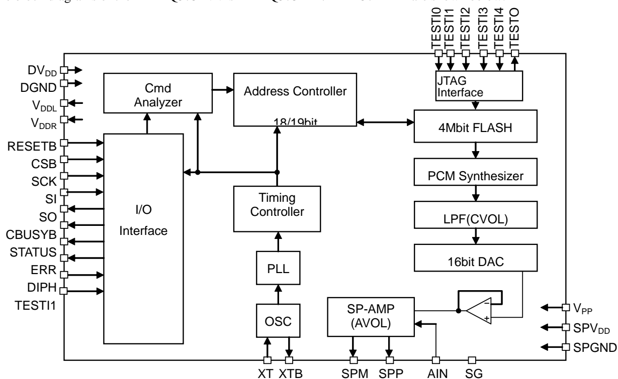
Block Diagram of ML22Q573-NNN/ML22Q573-xxx
