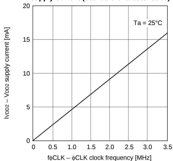
Operational frequency characteristics of the V DD2 supply current (Standard characteristics)
