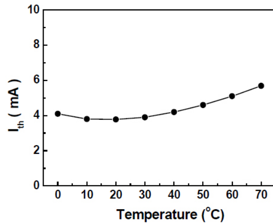
Threshold Current vs. Temperature
