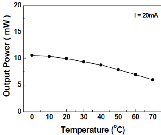
Optical Output Power vs. Temperature
