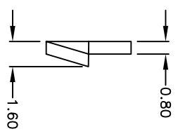
LOCK WASHER (2 PCS)
