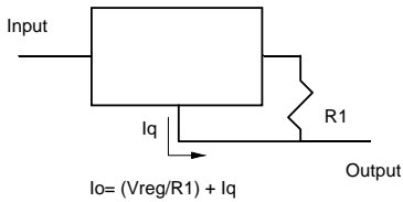
Current Regulator
