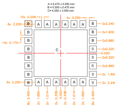
PCB Solder Mask Pattern
