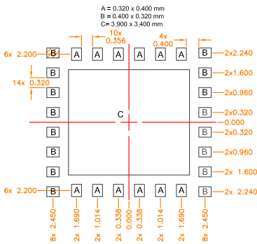
PCB Metal Land Pattern
