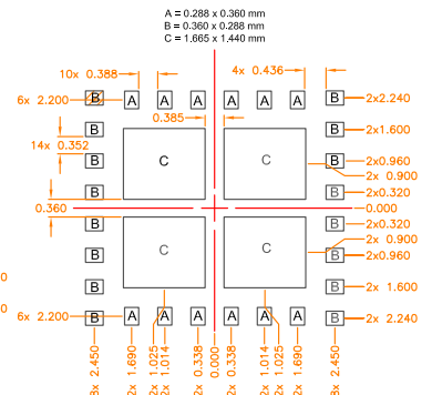
PCB Stencil Pattern
