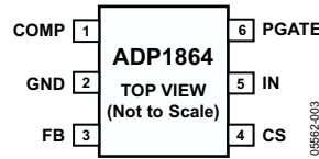
Figure 2. Pin Configuration
