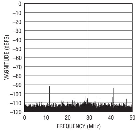
32k-Point FFT, f_{IN} = 70.3\text{MHz} , -1dBFS, 100Msps
