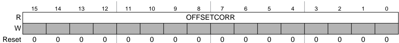
Figure 13-29. Offset Correction Value Register (OFCORVR)
