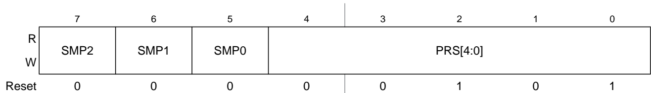
Figure 24-7. ATD Control Register 4 (ATDCTL4)
