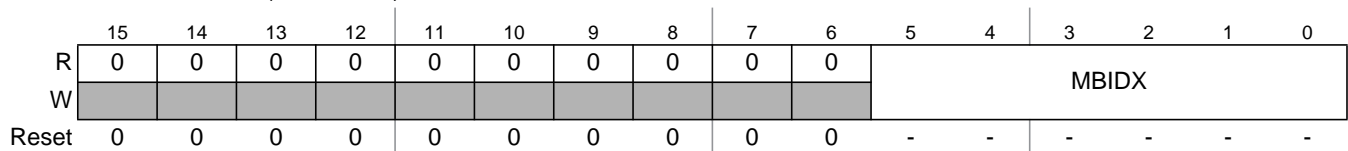
Figure 13-99. Message Buffer Index Registers (MBIDXRn)
