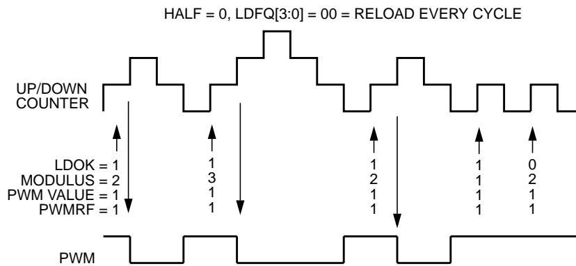
Figure 20-69. Full-Cycle Center-Aligned Modulus Loading
