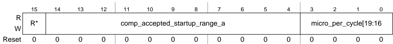
Figure 13-87. Protocol Configuration Register 22 (PCR22)
