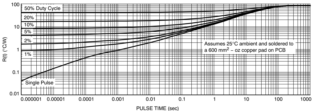
Figure 8. Thermal Characteristics
