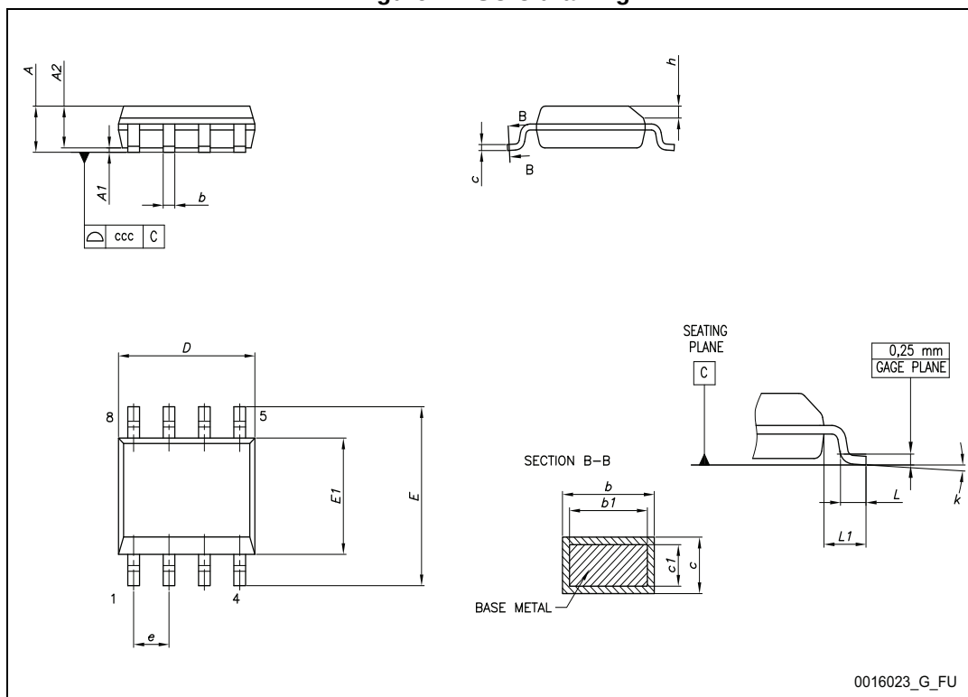
Figure 12. SO-8 drawing
