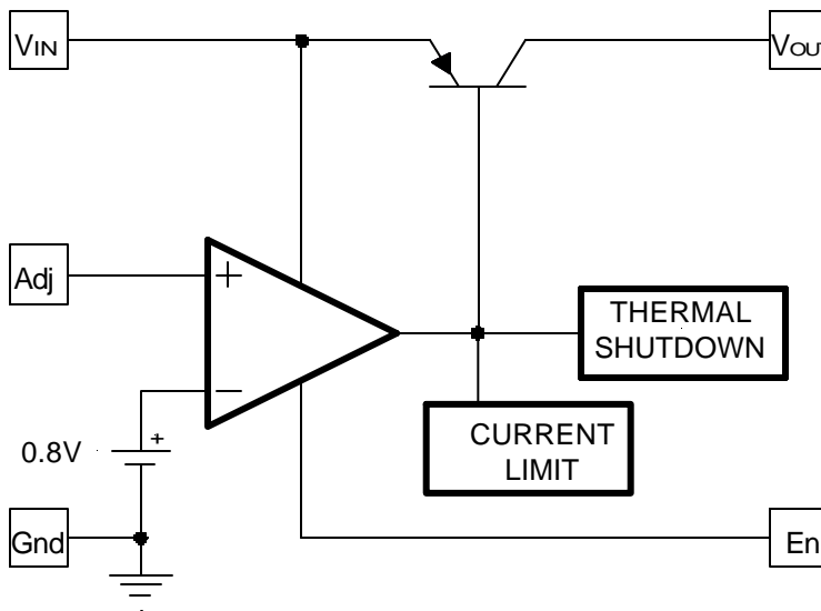
Figure 2 - APU8836 Adjustable output block diagram.
