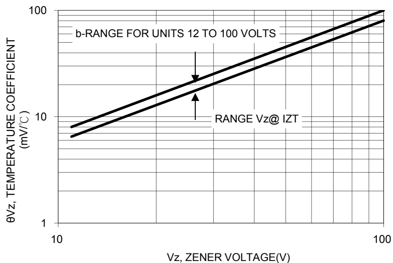
FIG.8 TEMPERATURE COEFFICIENTS
