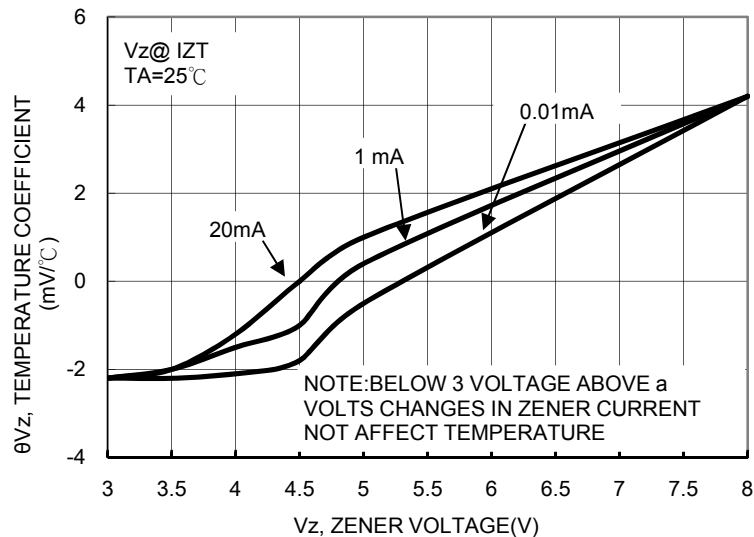
FIG. 9 EFFECT OF ZENER CURRENT
