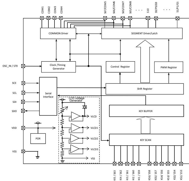
Figure 2. Block Diagram
