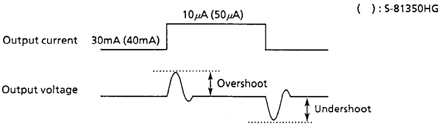
Figure 12 Ringing waveform
