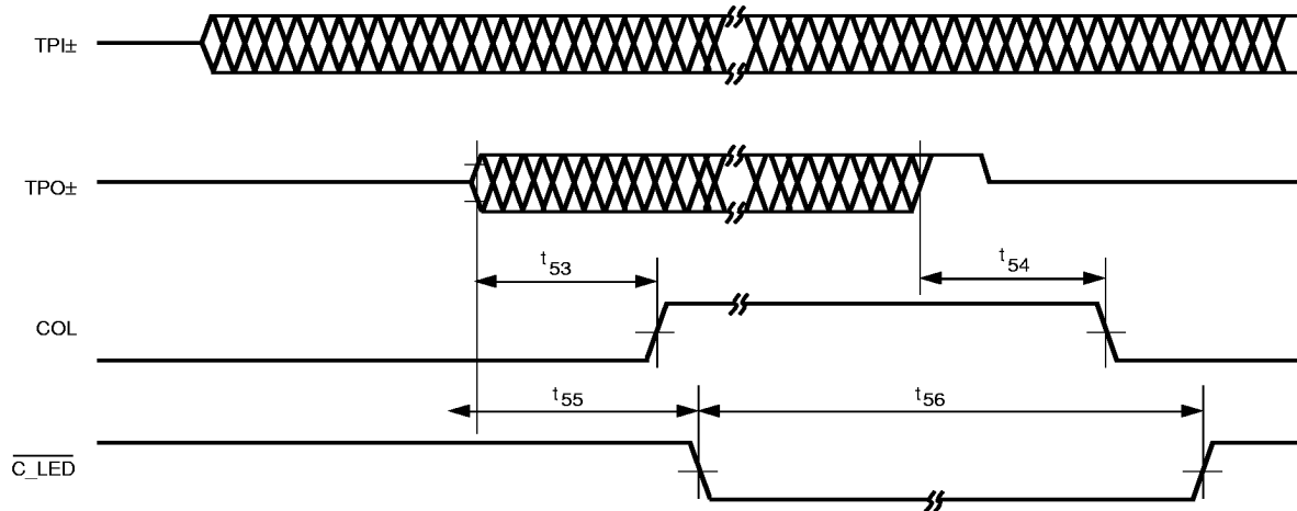
Figure 25. Collision Timing, Transmit
