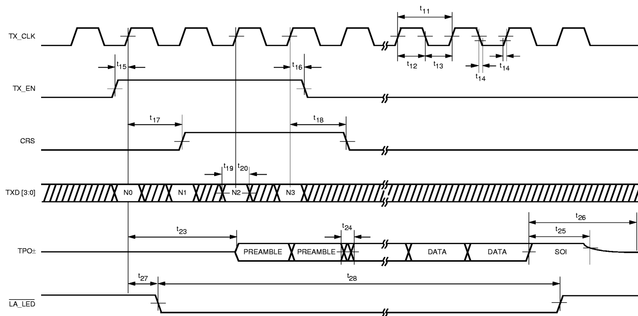
Figure 18. Transmit Timing - 10 Mbps
