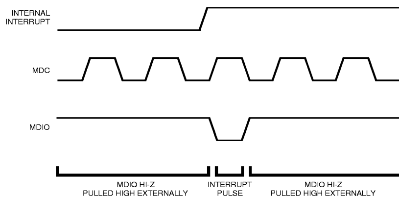
a.) Interrupt Happens During Idle.
