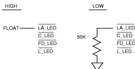
Figure 15. Serial Device Port Address Selection
