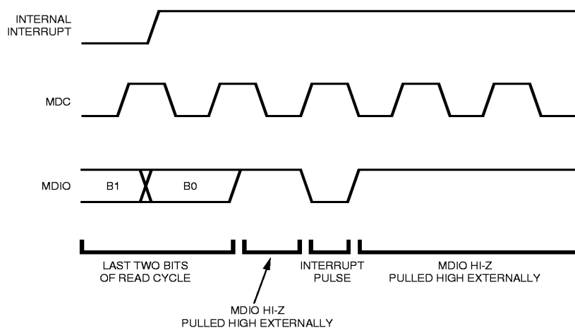
b.) Interrupt Happens During Read Cycle.
