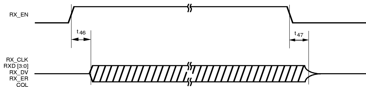
Figure 23. RX_EN Timing
