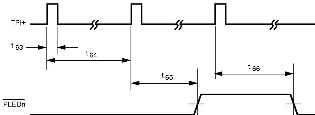
b.) Receive NLP
