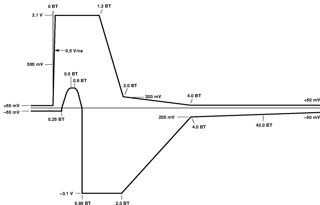
Figure 7. Link Pulse Output Voltage Template _ NLP, FLP
