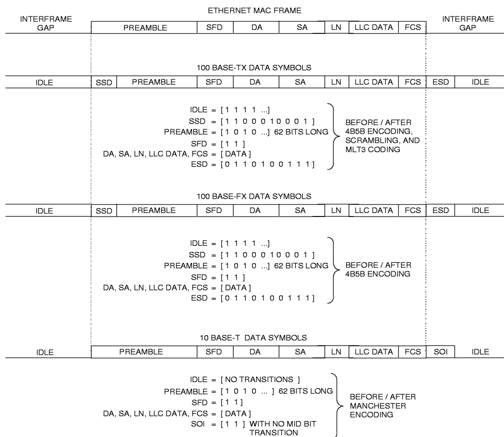
Figure 2. TX/10BT Frame Format
