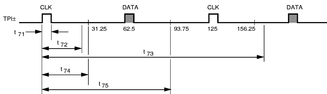
b.) Receive FLP
