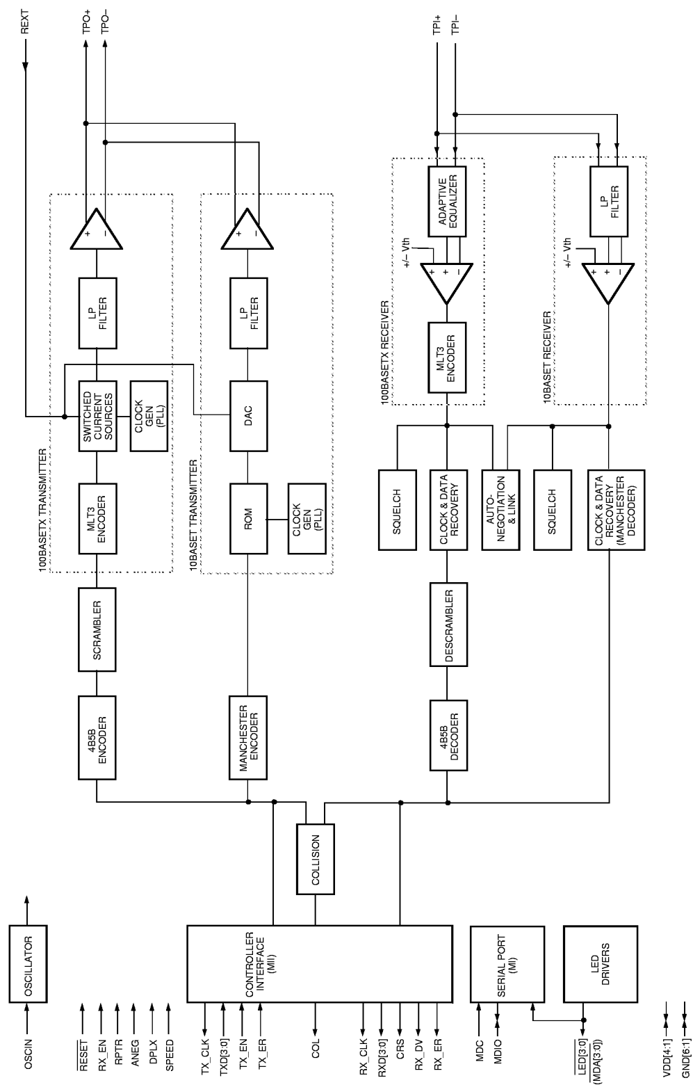
Figure 1. 80225 Block Diagram
