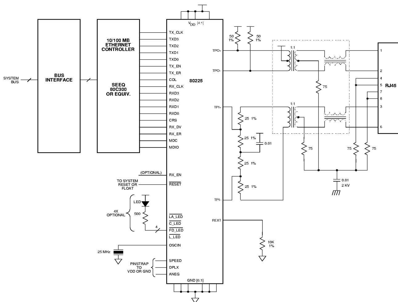
Figure 11. Typical Network Interface Card Schematic Using 80225
