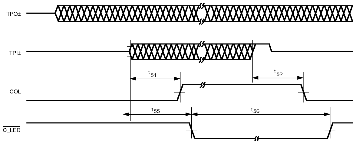
Figure 24. Collision Timing, Receive
