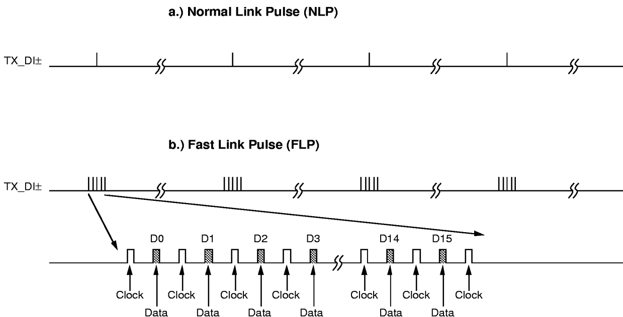
Figure 8. NLP vs. FLP Link Pulse
