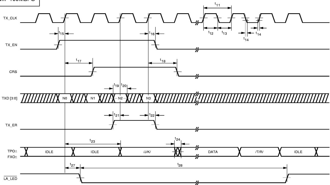
Figure 17. Transmit Timing - 100 Mbps
