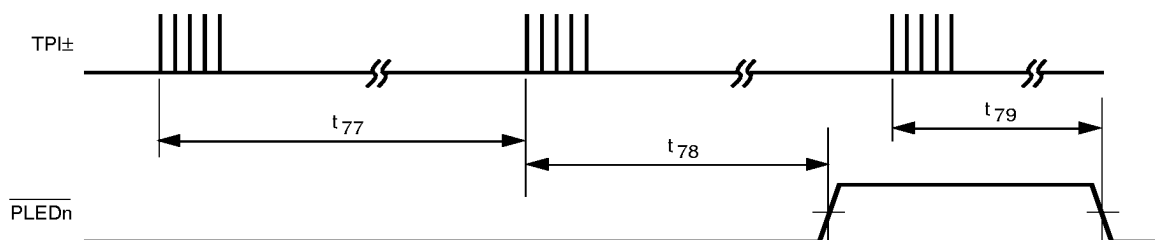
c.) Receive FLP Burst
