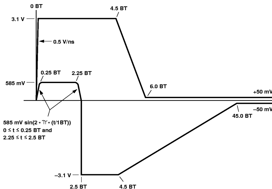
Figure 6. SOI Output Voltage Template - 10 Mbps
