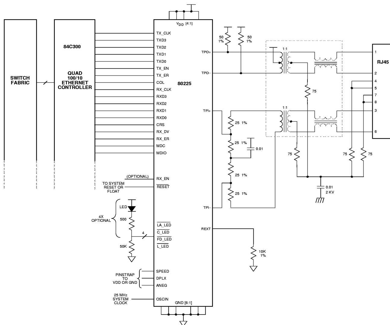
Figure 12. Typical Switching Port Schematic Using 80225
