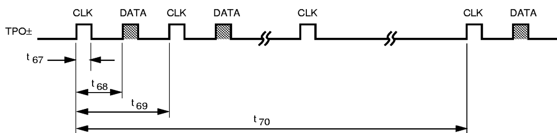
a.) Transmit FLP and Transmit FLP Burst
