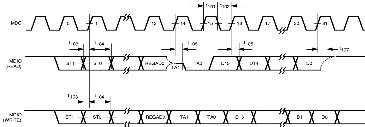
Figure 31. MI Serial Port Timing
