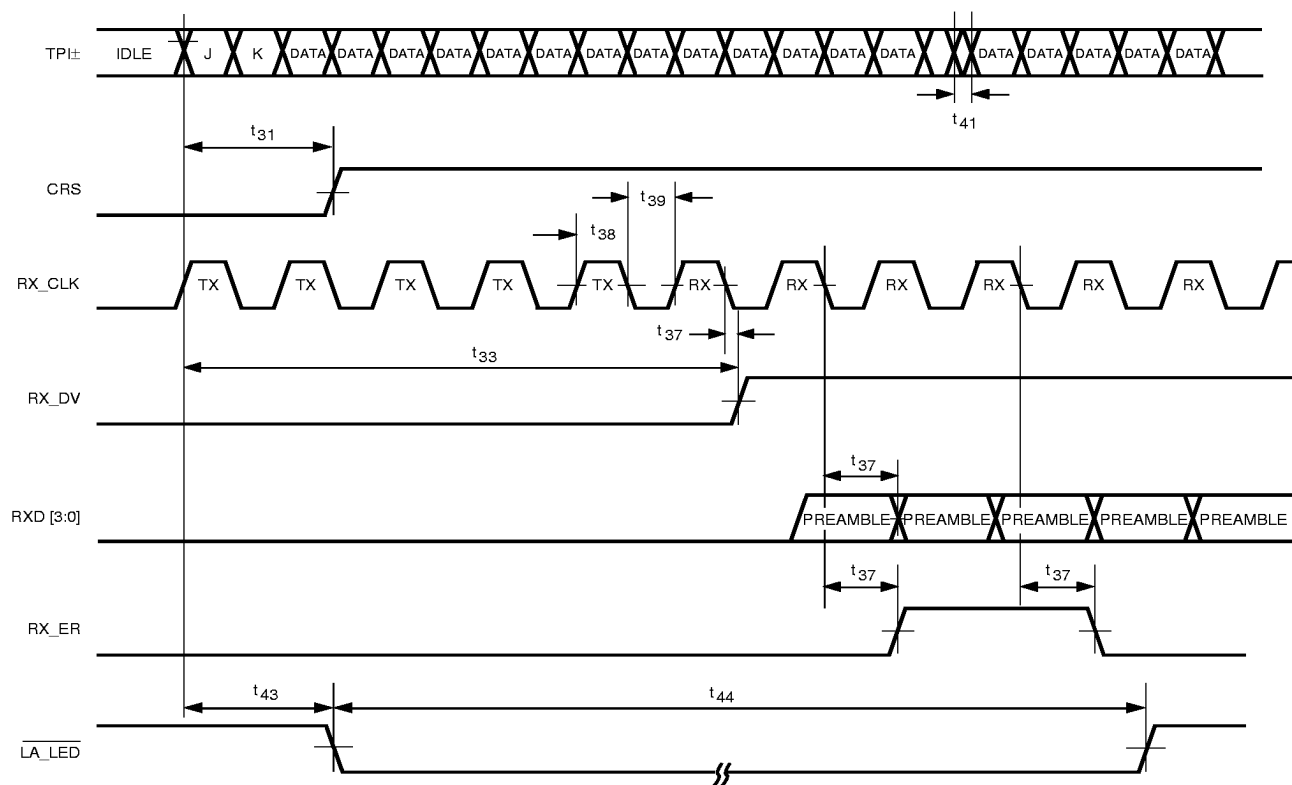
Figure 19. Receive Timing, Start of Packet - 100 Mbps
