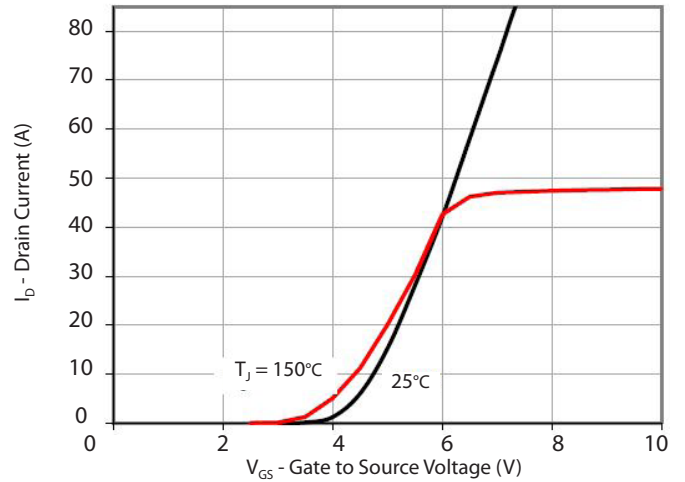
Transfer Characteristics
