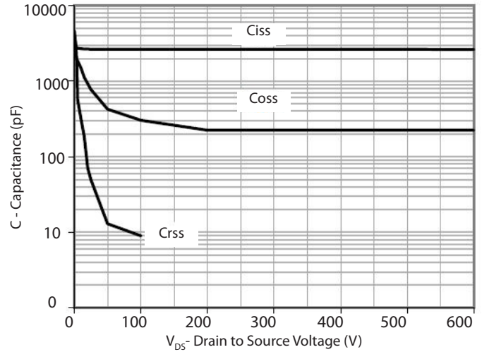
Capacitance
