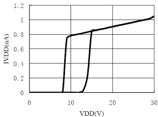
IVDD vs VDD
