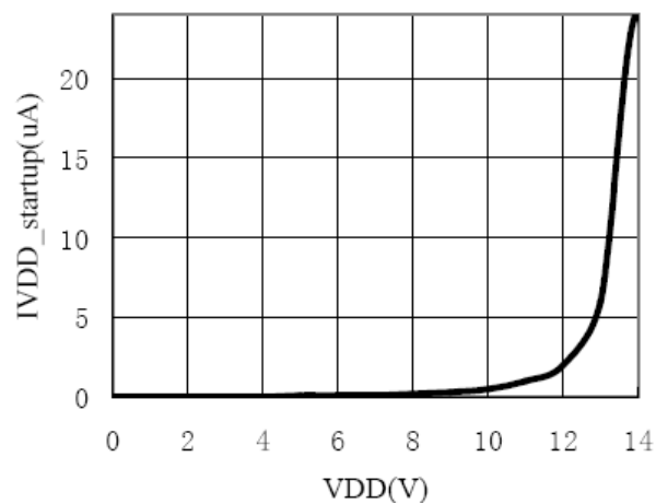
IVDD_startup vs VDD
