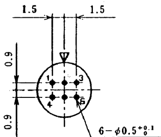
Size 7, 6 conductors
