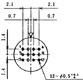
Size 9, 12 conductors
