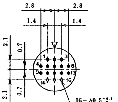
Size 9, 16 conductors
