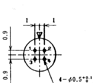
Size 7, 4 conductors
