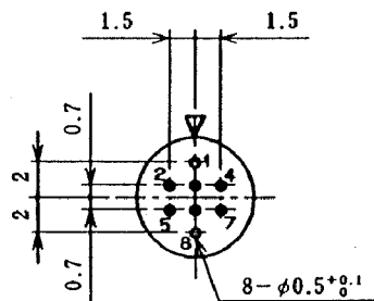
Size 7, 8 conductors
