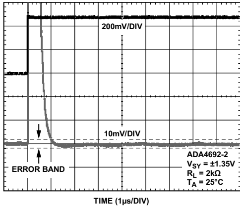
Figure 51. Positive Settling Time to 0.1%
