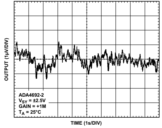
Figure 43. 0.1 Hz to 10 Hz Noise
