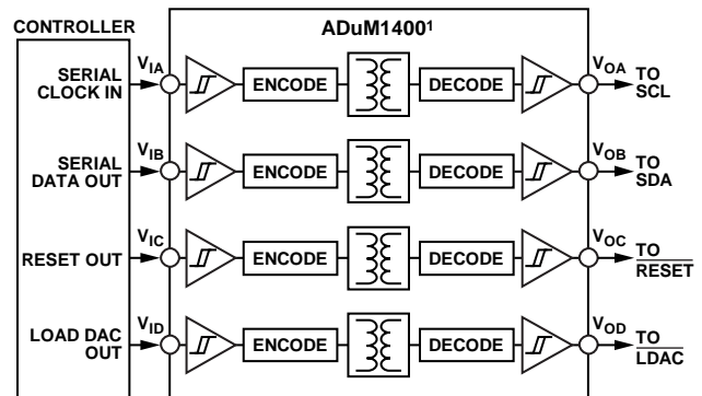
Figure 60. Isolated Interface
