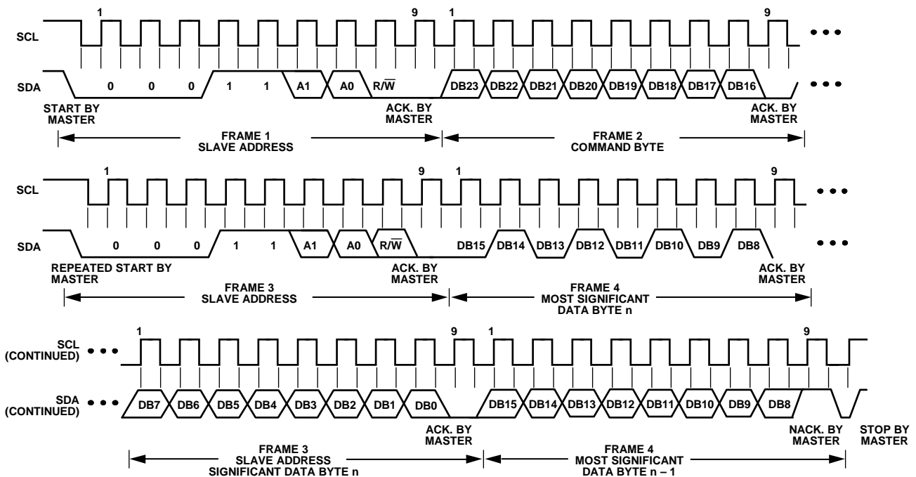
Figure 52. I 2 C Read Operation
