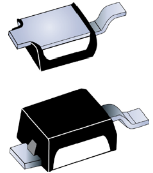
Powermite 1 (DO-216AA) Package
