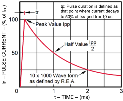
FIGURE 1 Pulse Waveform for 10/1000 \mu s Exponential Surge
