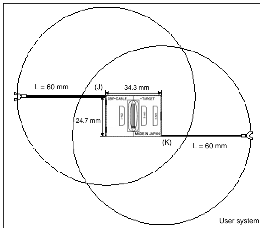
Figure 2-7 Where GND Wire Can Be Connected
