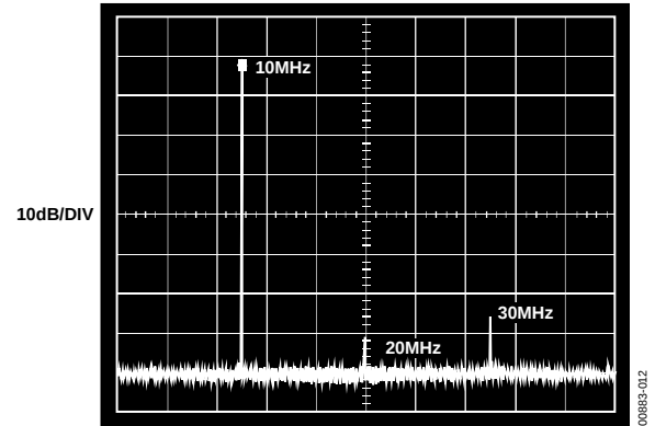
Figure 12. Harmonic Distortion at 10 MHz; 10 dBm Input to X or Y Channels, R_L = 150\ \Omega , C_L \leq 5\ \text{pF}
