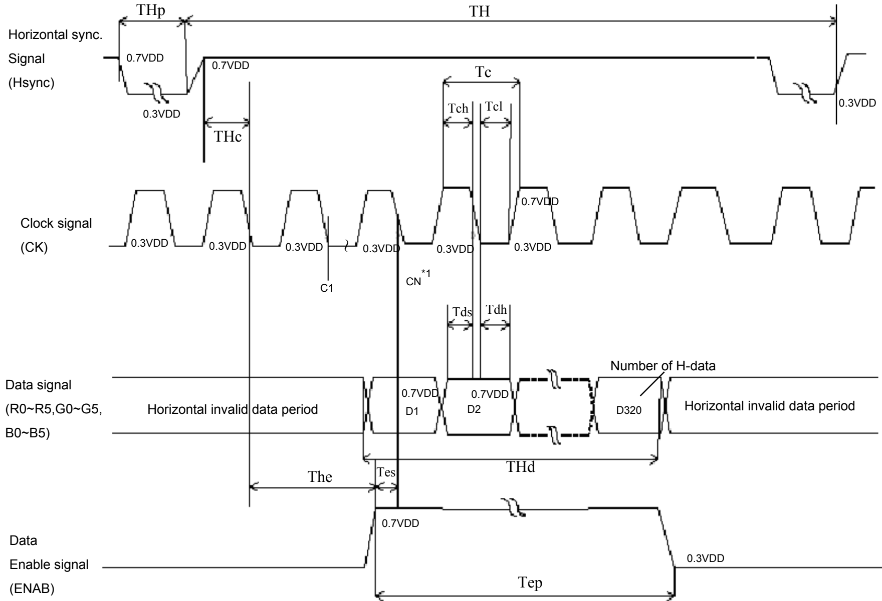
11-2) Timing Diagram :
