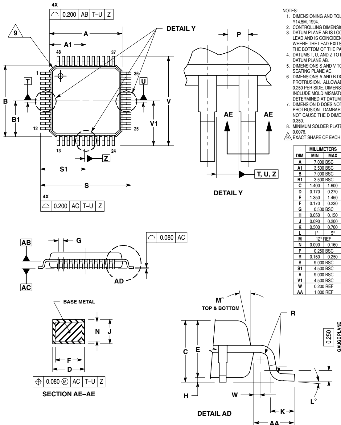
Figure 23-1. 48-Pin LQFP (Case #932)
