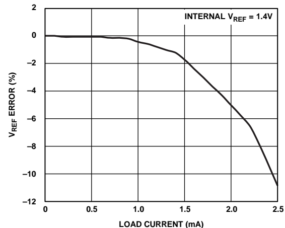
Figure 53. V_{REF} Error (Internal V_{REF} = 1.4 \text{ V} ) vs. Load Current
