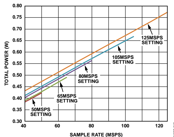
Figure 63. Total Power vs. f_{\text{SAMPLE}} for f_{\text{IN}} = 9.7 \text{ MHz} , Four Channels ( V_{\text{REF}} = 1.0 \text{ V} )
