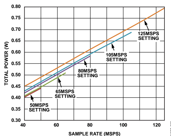
Figure 62. Total Power vs. f_{\text{SAMPLE}} for f_{\text{IN}} = 9.7 \text{ MHz} , Four Channels ( V_{\text{REF}} = 1.4 \text{ V} )
