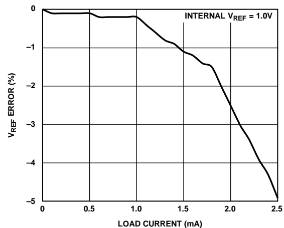
Figure 52. V_{REF} Error (Internal V_{REF} = 1.0 \text{ V} ) vs. Load Current
