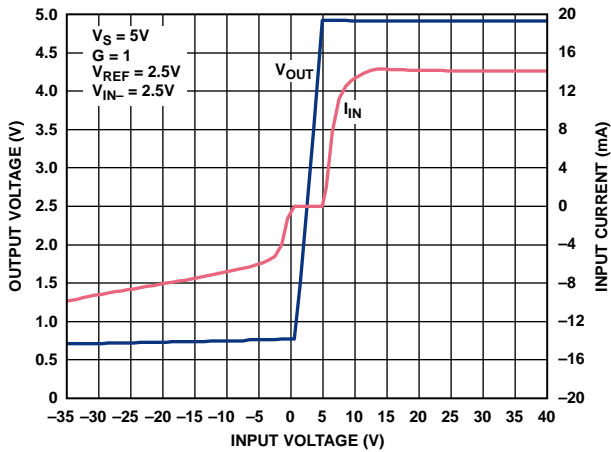
Figure 16. Input Overvoltage Performance; G = 1 , V_S = 5V
