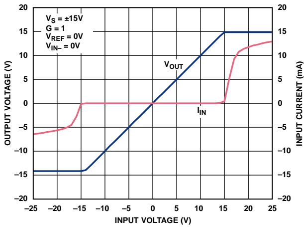
Figure 17. Input Overvoltage Performance; G = 1 , V_S = \pm 15V
