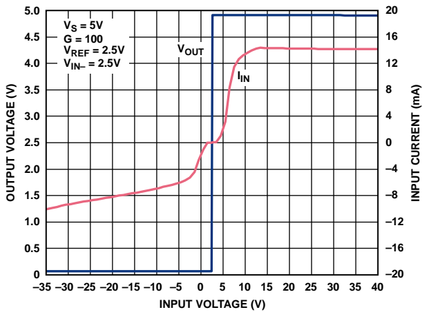
Figure 18. Input Overvoltage Performance; G = 100 , V_S = 5V
