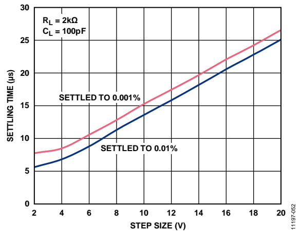
Figure 51. Settling Time vs. Step Size ( G = 1 )
