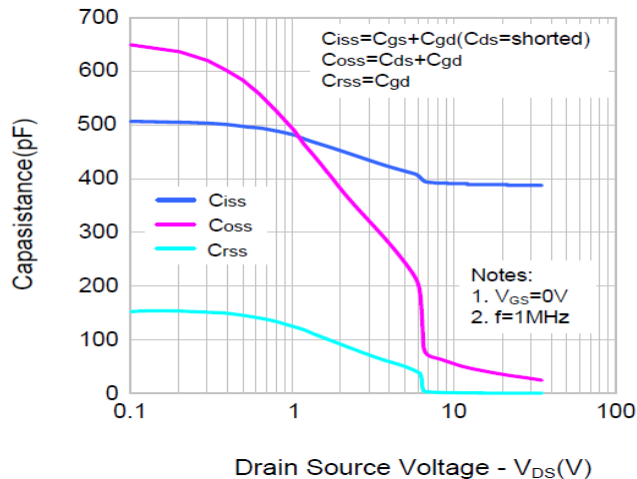
Figure 5. Capacitance Characteristics
