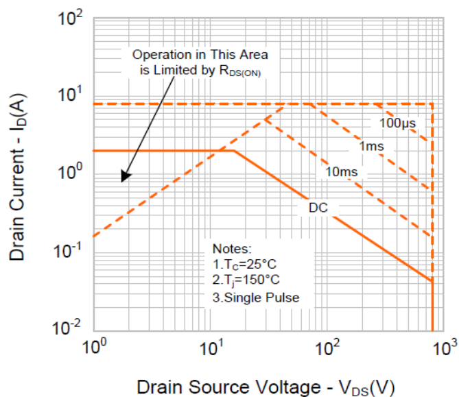
Figure 9 Max. Safe Operating Area
