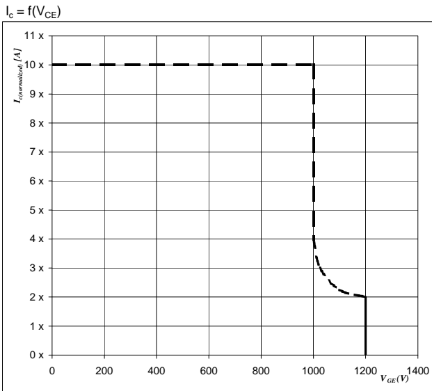
Figure 27 Output inverter IGBT
