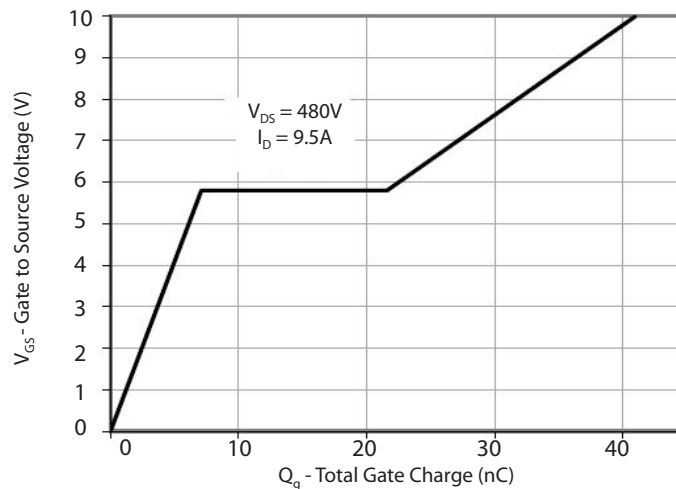
Gate Charge
