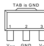
SOT-89 (Top View) APL5309
