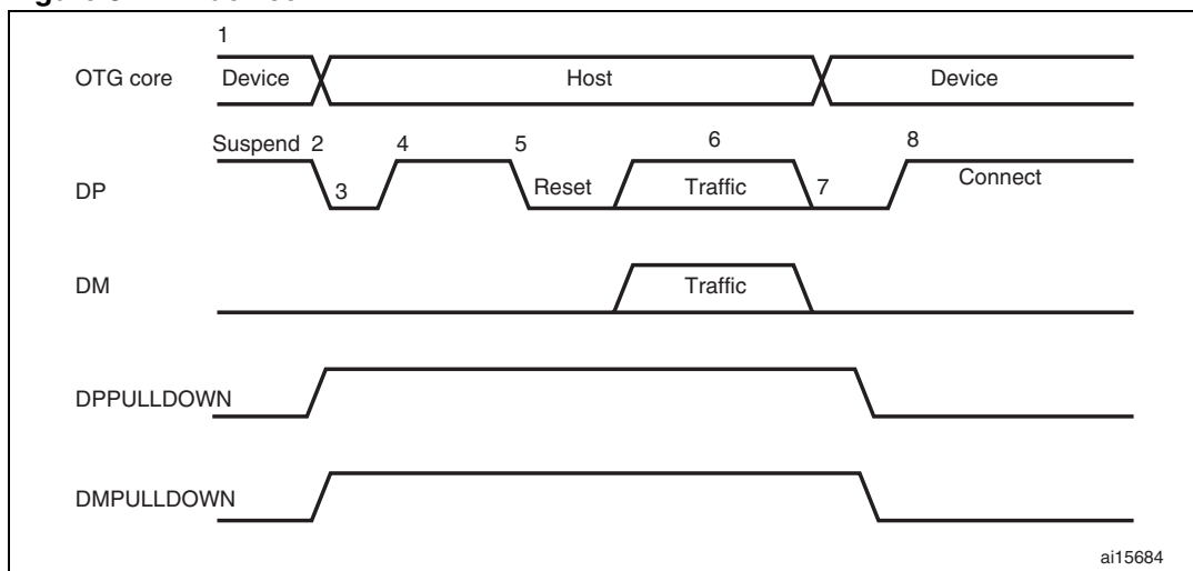
Figure 371. B-device HNP
