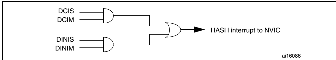
Figure 213. HASH interrupt mapping diagram
