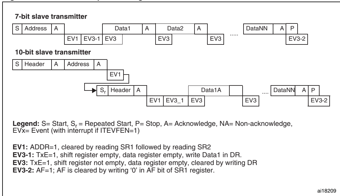
Figure 217. Transfer sequence diagram for slave transmitter
