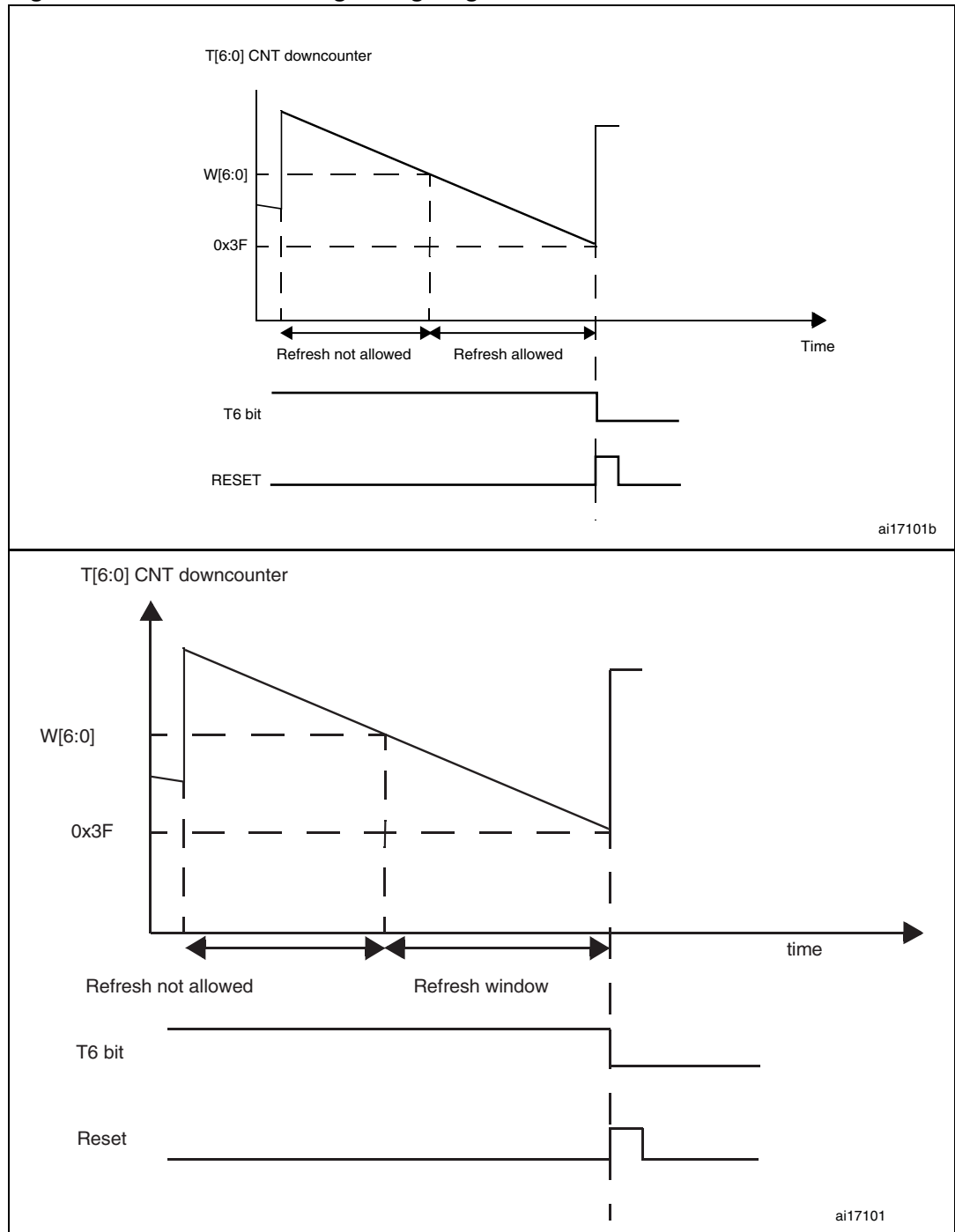
Figure 194. Window watchdog timing diagram
