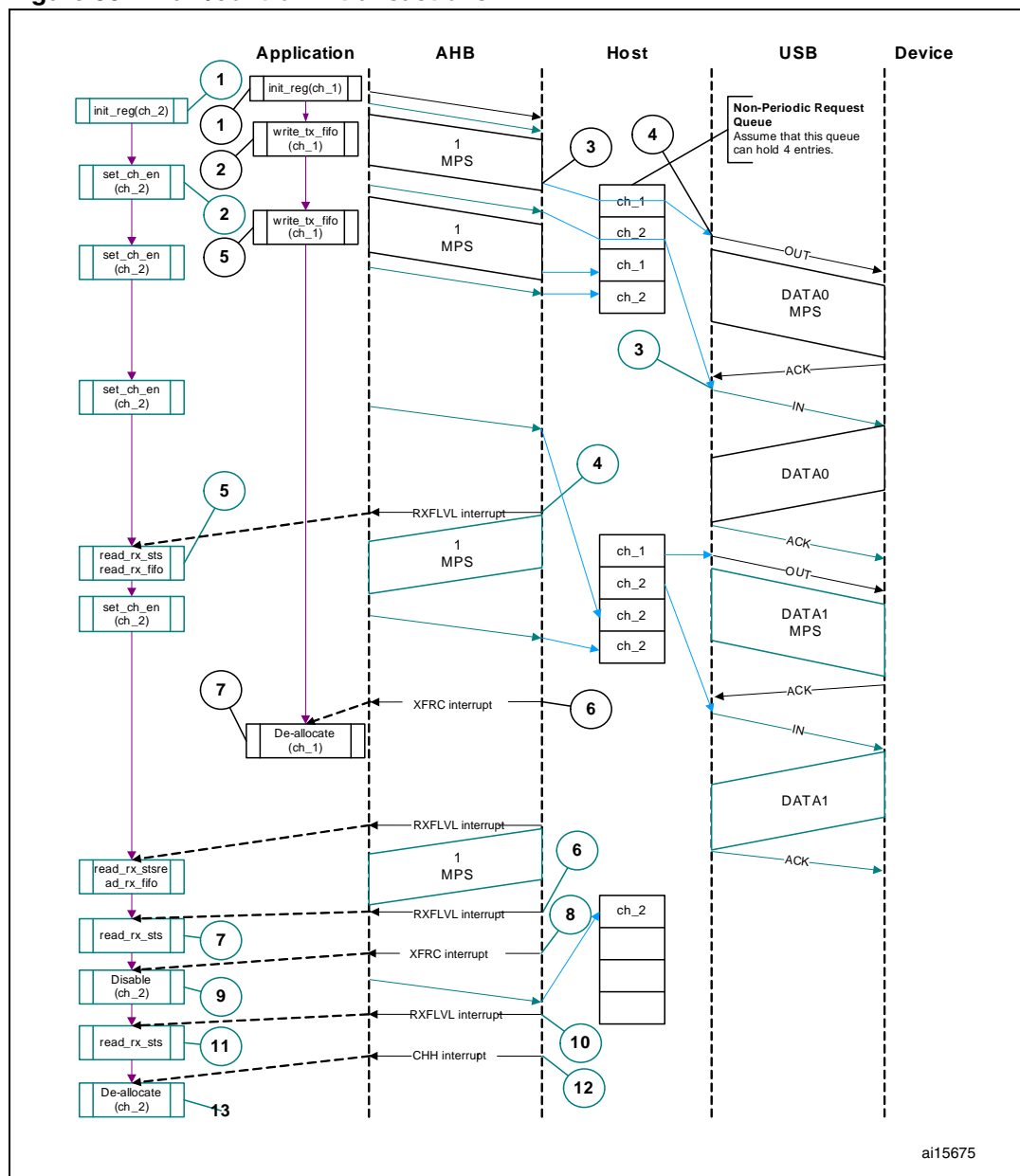
Figure 361. Bulk/control IN transactions
