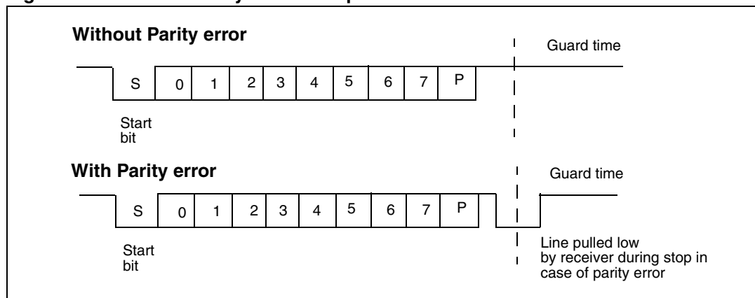
Figure 237. ISO 7816-3 asynchronous protocol
