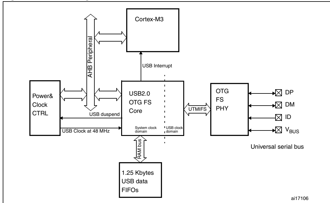
Figure 348. Block diagram
