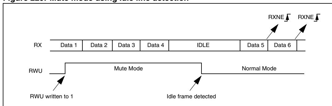
Figure 229. Mute mode using Idle line detection
