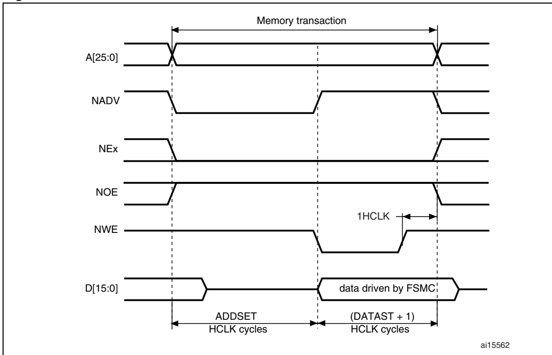
Figure 402. ModeB write accesses
