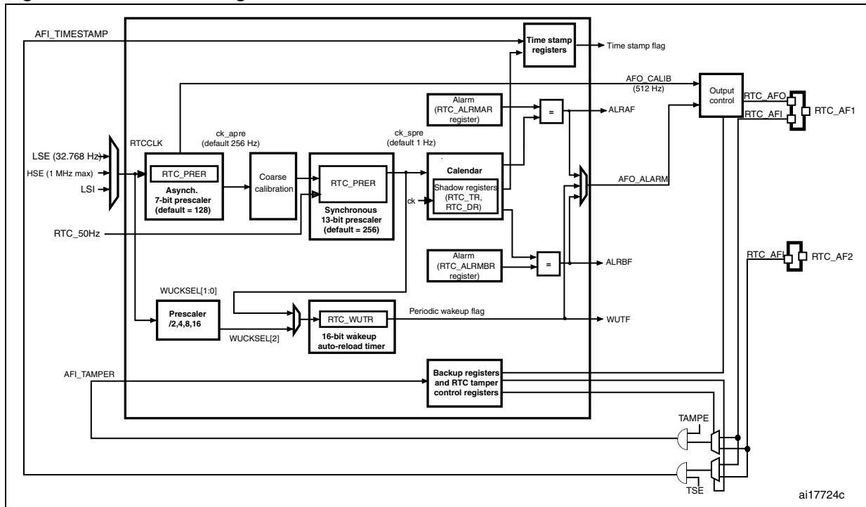
Figure 214. RTC block diagram
