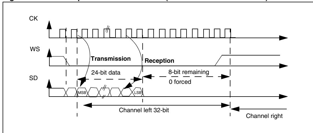
Figure 266. I 2 S Phillips standard waveforms (24-bit frame with CPOL = 0)
