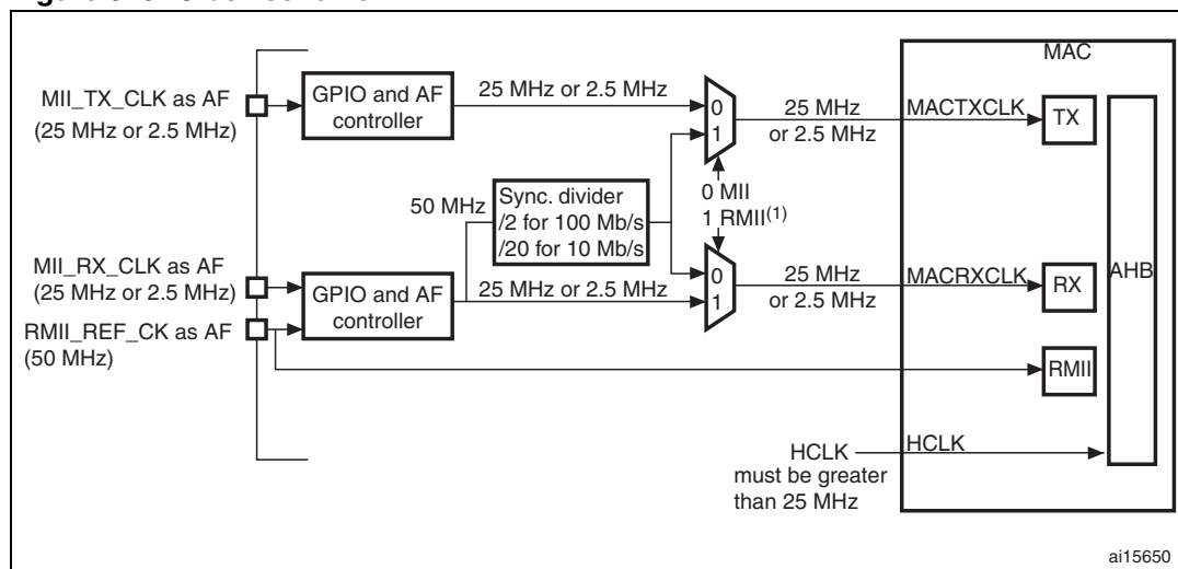
Figure 320. Clock scheme
