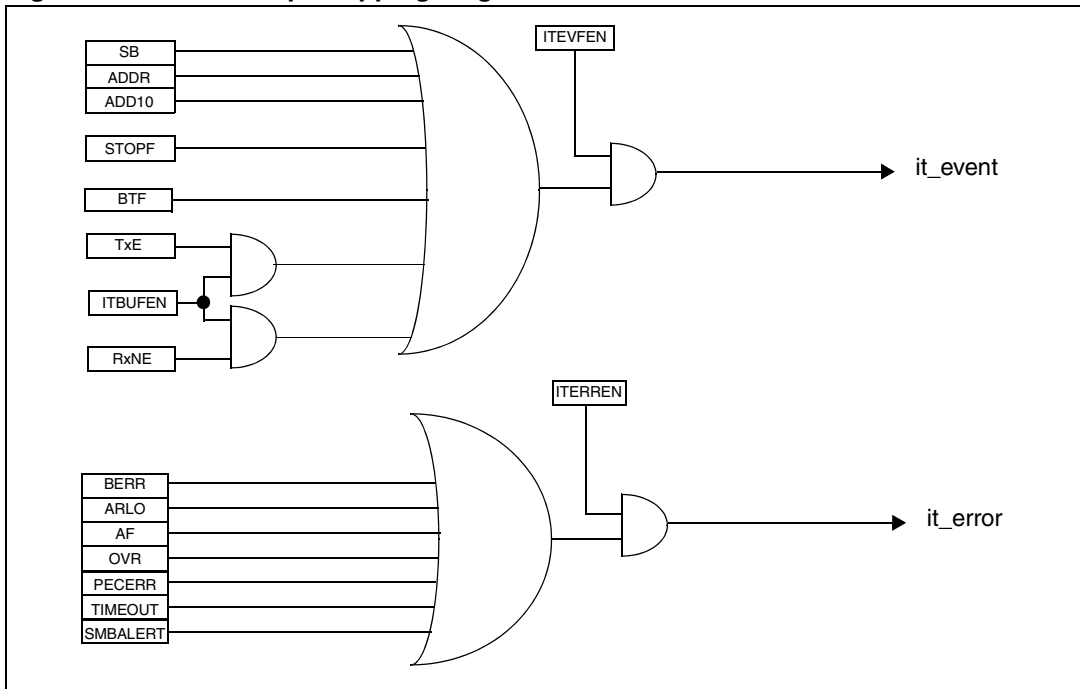
Figure 221. I 2 C interrupt mapping diagram
