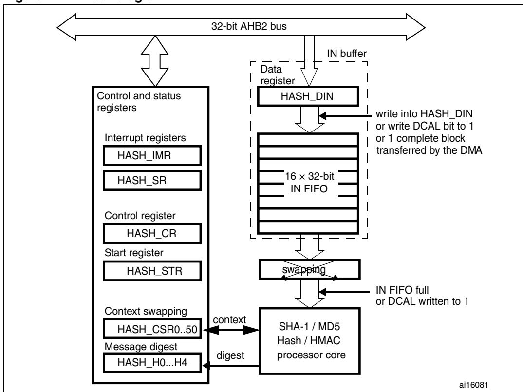
Figure 211. Block diagram
