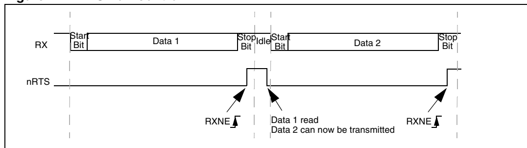
Figure 244. RTS flow control
