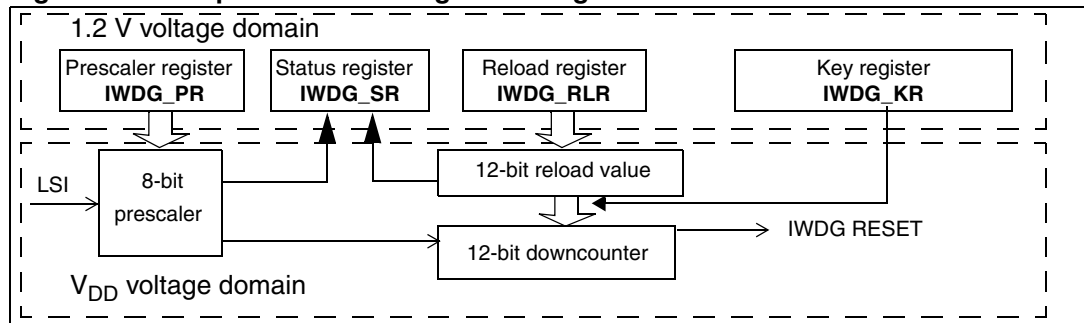
Figure 192. Independent watchdog block diagram
