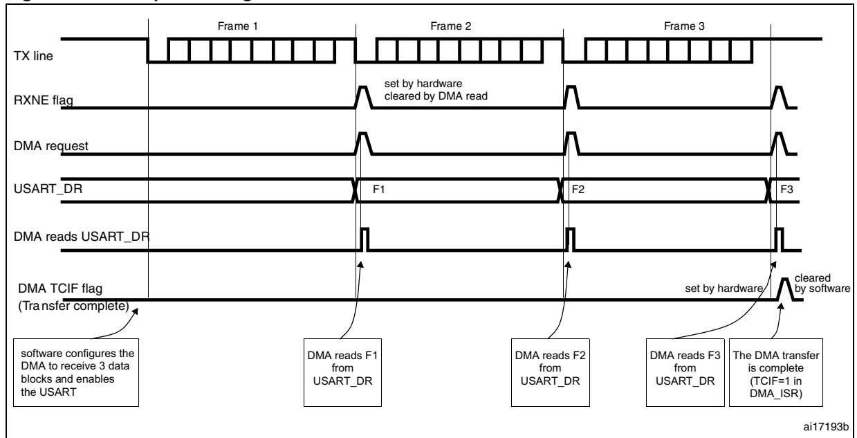
Figure 242. Reception using DMA
