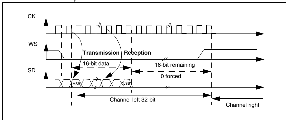
Figure 269. I 2 S Phillips standard (16-bit extended to 32-bit packet frame with CPOL = 0)
