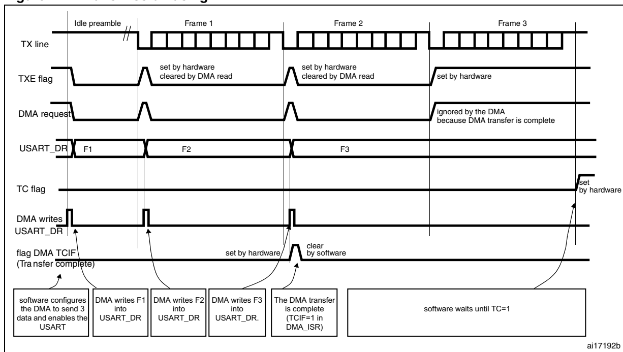
Figure 241. Transmission using DMA
