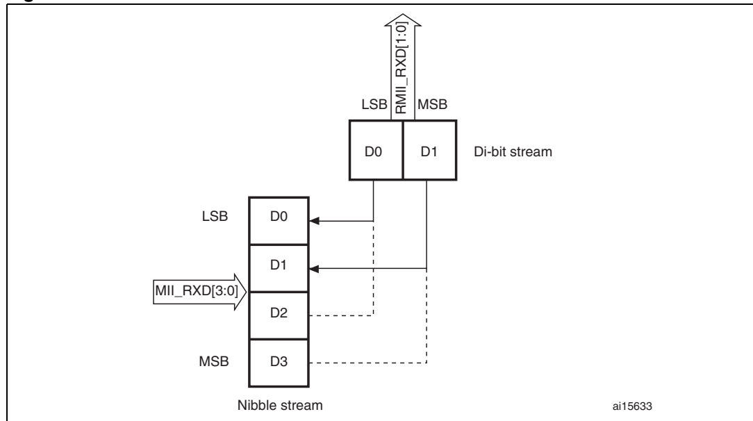
Figure 328. Receive bit order
