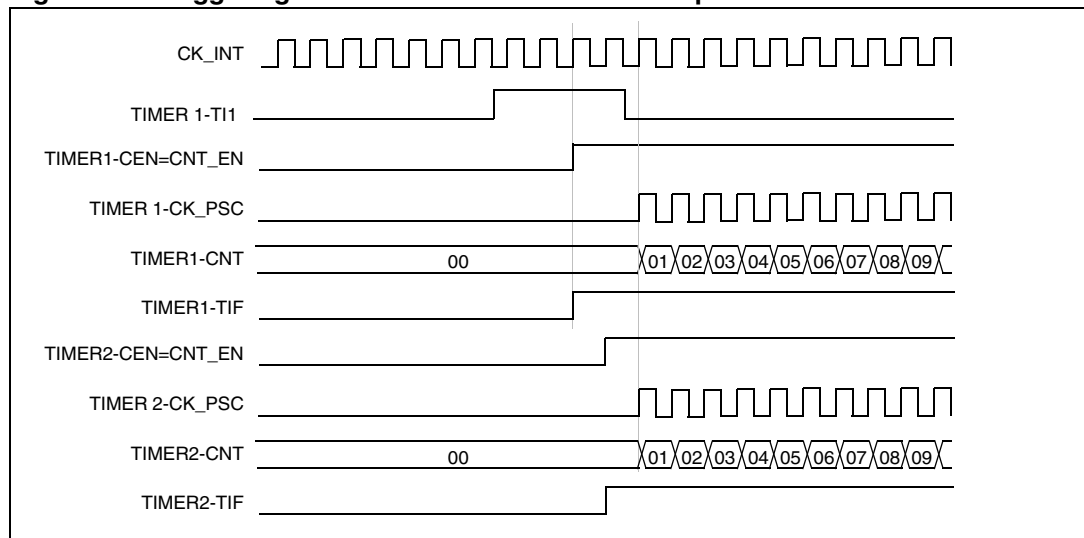
Figure 158. Triggering timer 1 and 2 with timer 1 TI1 input
