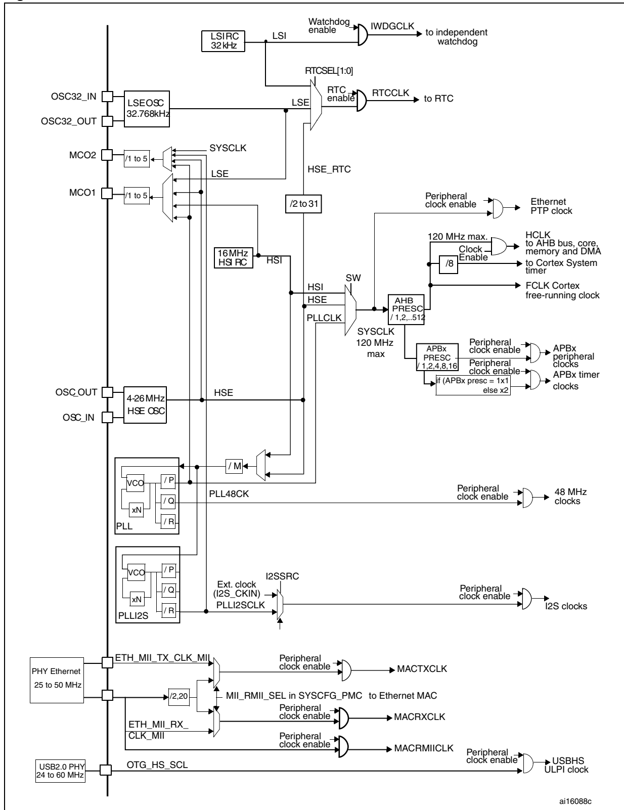
Figure 9. Clock tree
