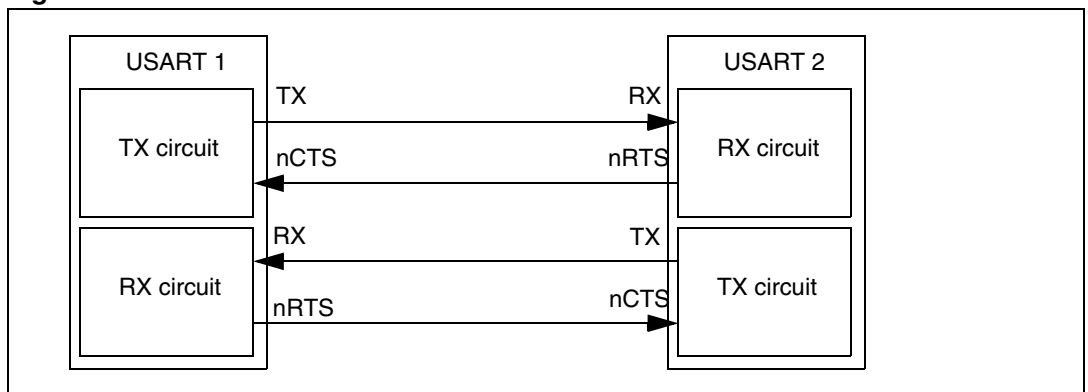
Figure 243. Hardware flow control between 2 USARTs
