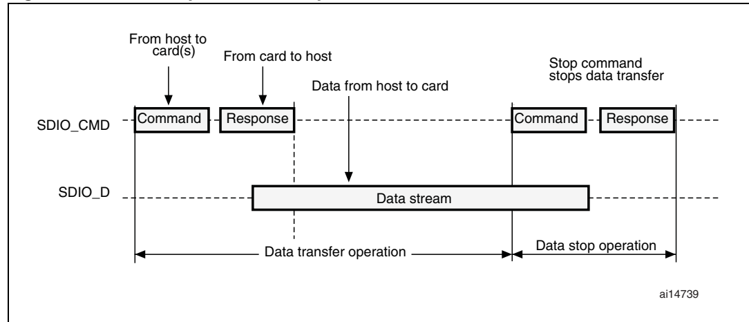
Figure 288. SDIO sequential write operation
