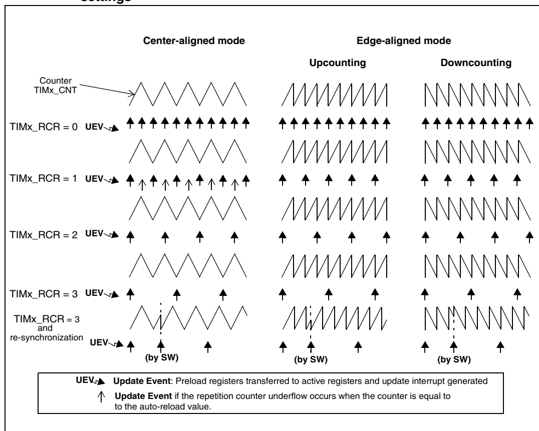
Figure 85. Update rate examples depending on mode and TIMx_RCR register settings
