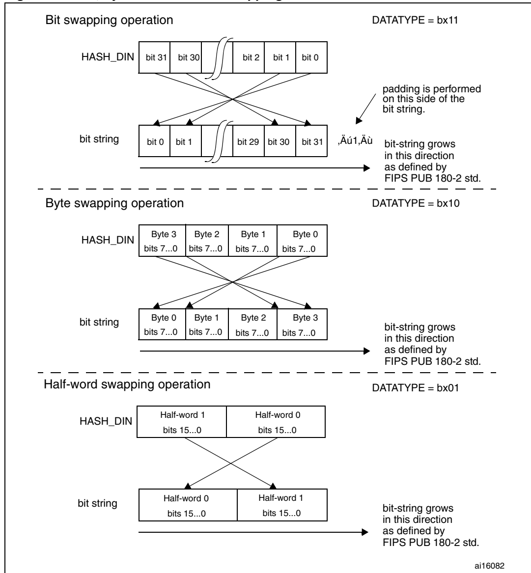
Figure 212. Bit, byte and half-word swapping
