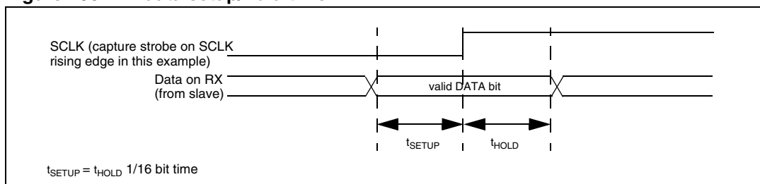
Figure 236. RX data setup/hold time
