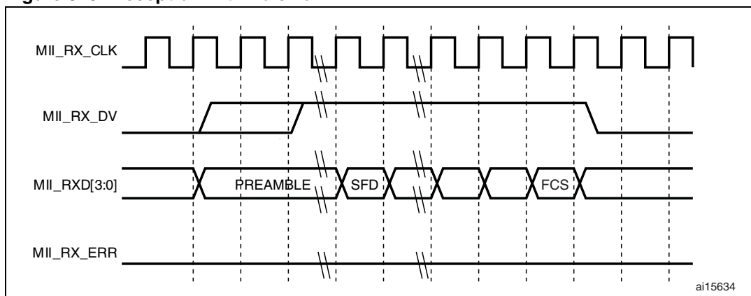
Figure 329. Reception with no error
