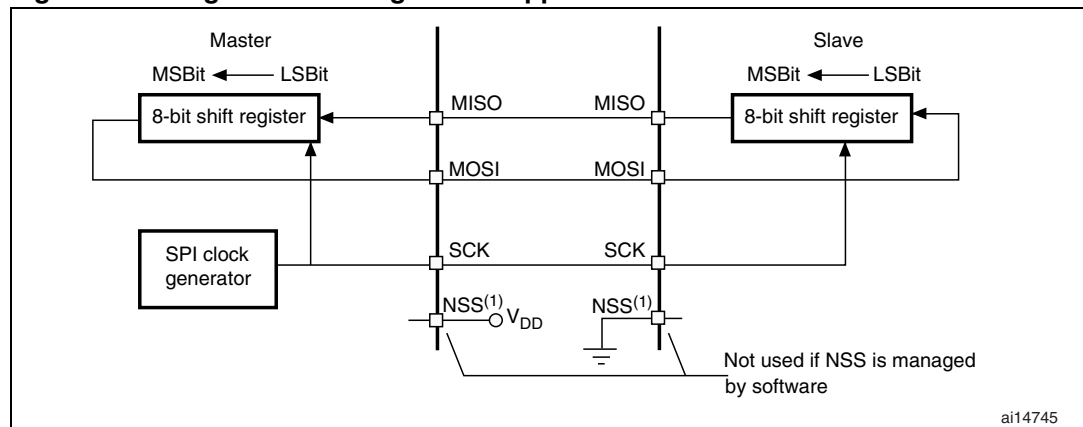
Figure 248. Single master/ single slave application
