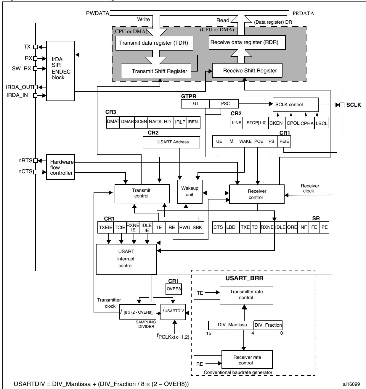
Figure 222. USART block diagram
