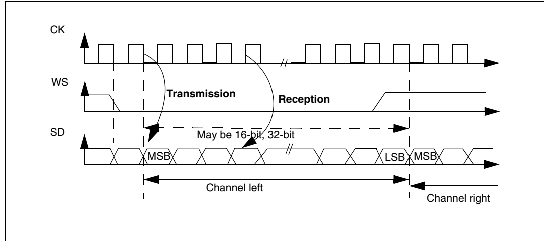
Figure 265. I 2 S Phillips protocol waveforms (16/32-bit full accuracy, CPOL = 0)
