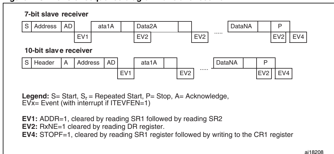
Figure 218. Transfer sequence diagram for slave receiver
