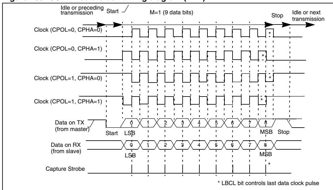
Figure 235. USART data clock timing diagram (M=1)
