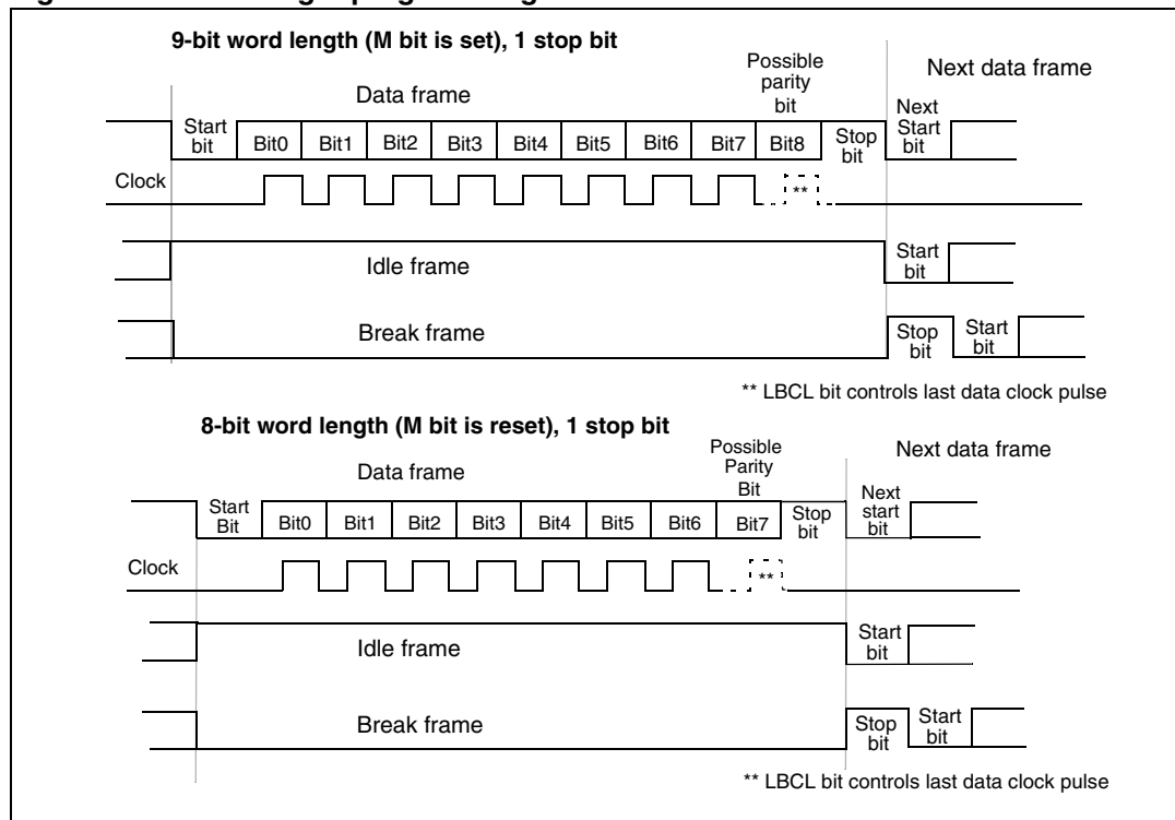
Figure 223. Word length programming
