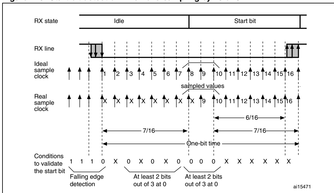
Figure 226. Start bit detection when oversampling by 16 or 8
