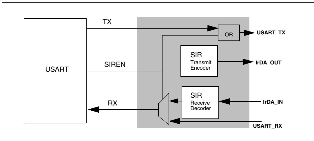
Figure 239. IrDA SIR ENDEC- block diagram
