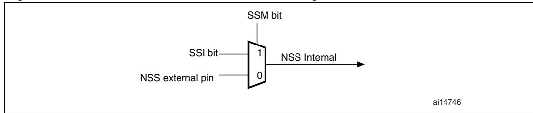
Figure 249. Hardware/software slave select management
