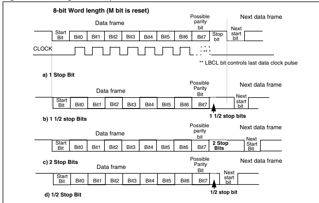
Figure 224. Configurable stop bits
