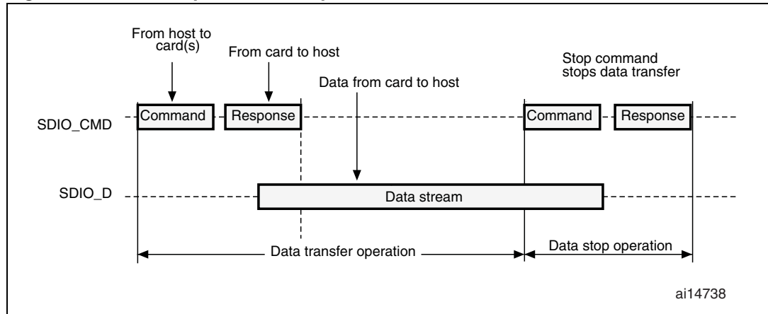
Figure 287. SDIO sequential read operation
