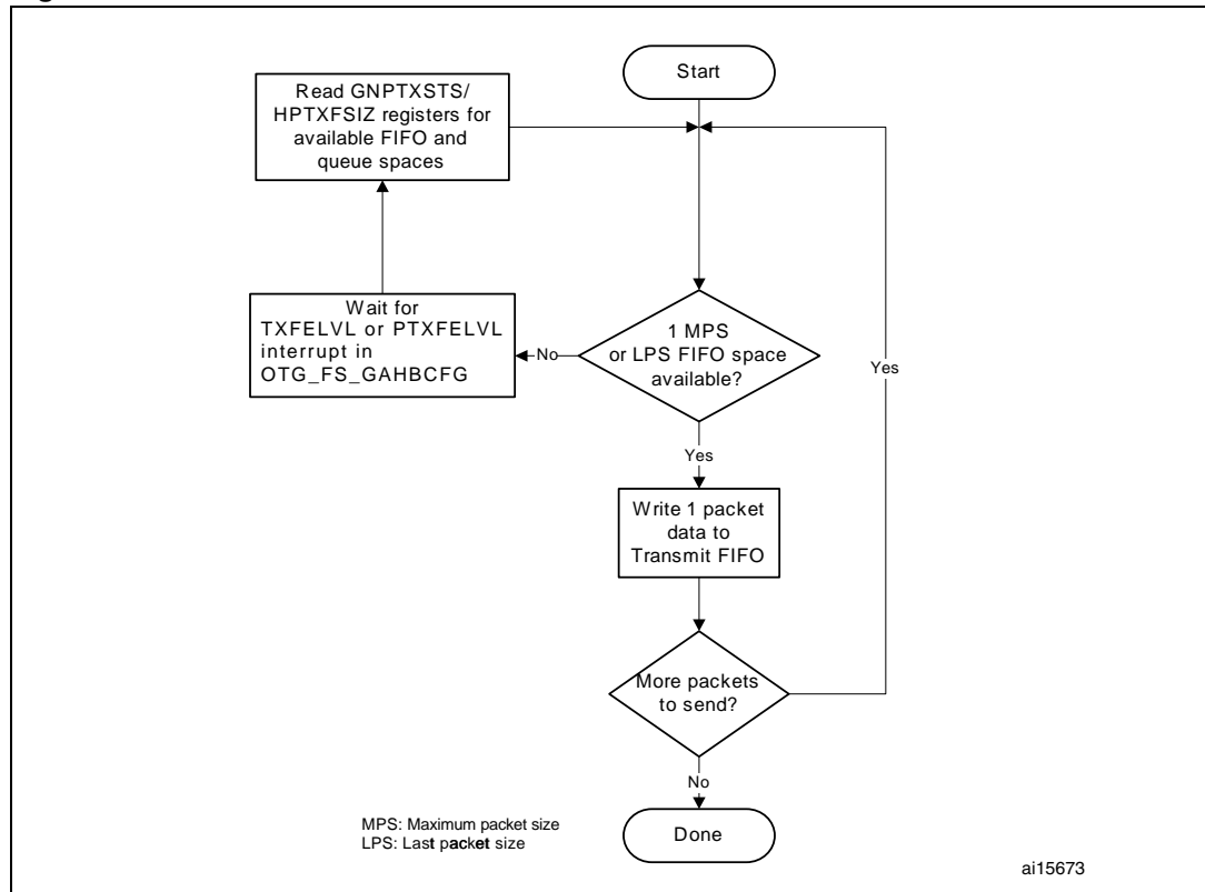
Figure 376. Transmit FIFO write task
