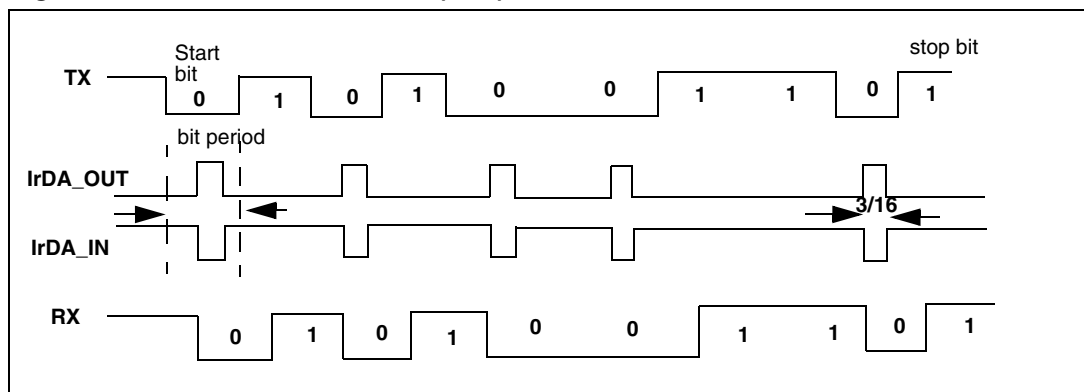
Figure 240. IrDA data modulation (3/16) -Normal mode
