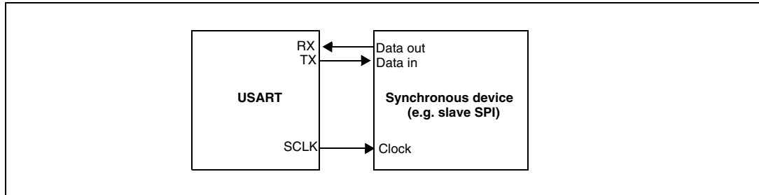
Figure 233. USART example of synchronous transmission
