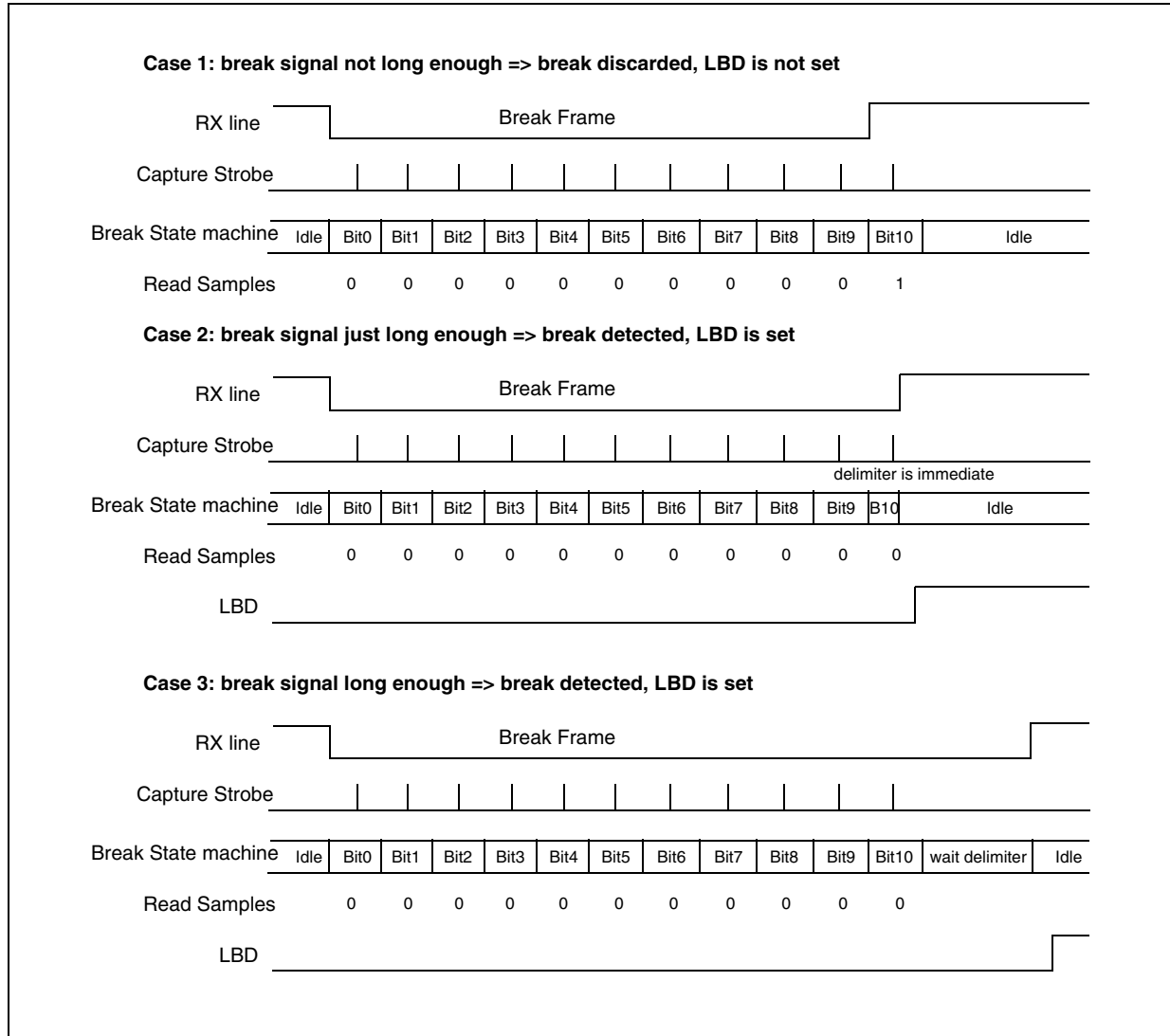
Figure 231. Break detection in LIN mode (11-bit break length - LBDL bit is set)
