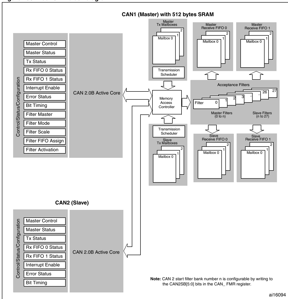
Figure 298. Dual CAN block diagram
