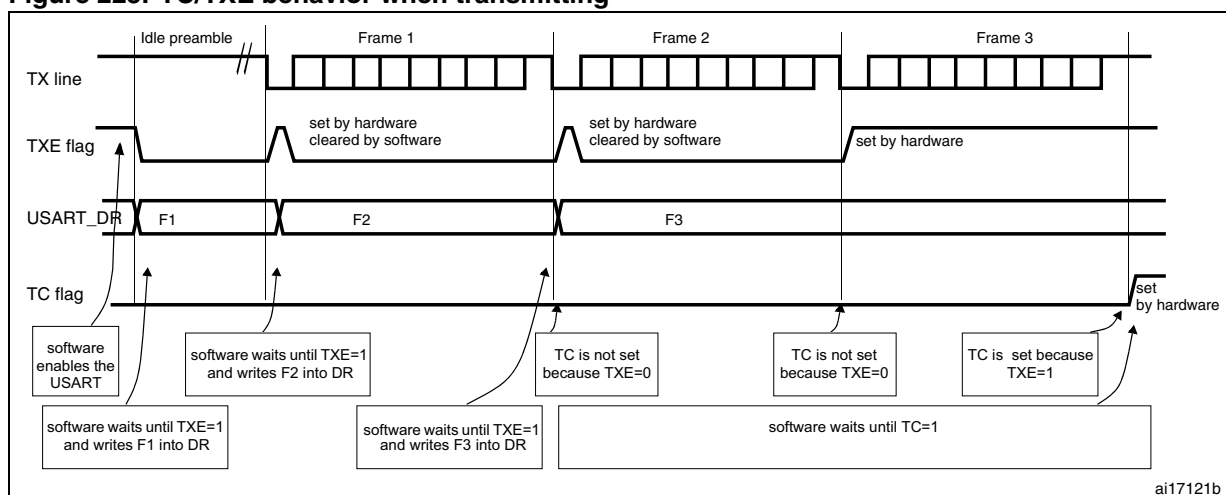
Figure 225. TC/TXE behavior when transmitting
