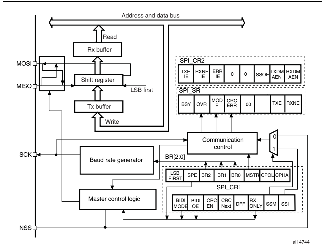
Figure 247. SPI block diagram
