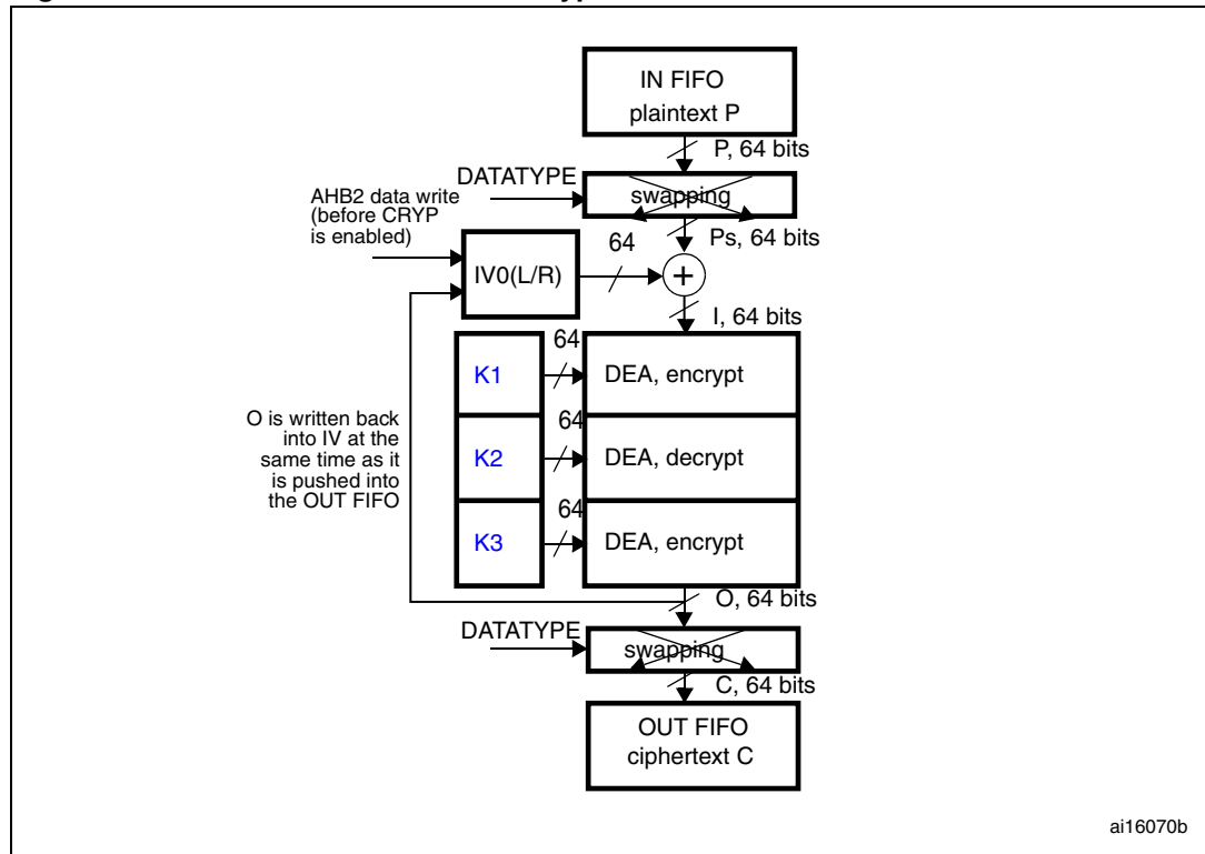
Figure 198. DES/TDES-CBC mode encryption
