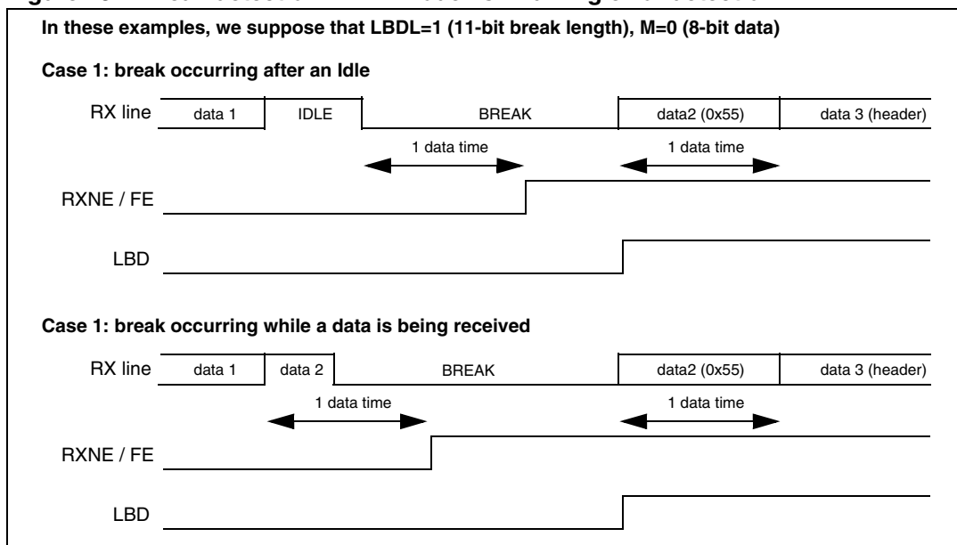
Figure 232. Break detection in LIN mode vs. Framing error detection
