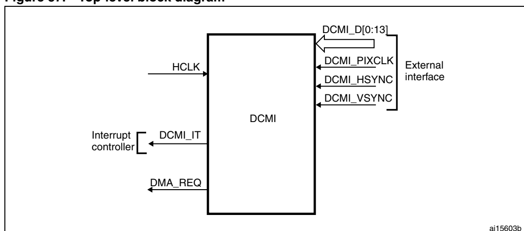
Figure 57. Top-level block diagram
