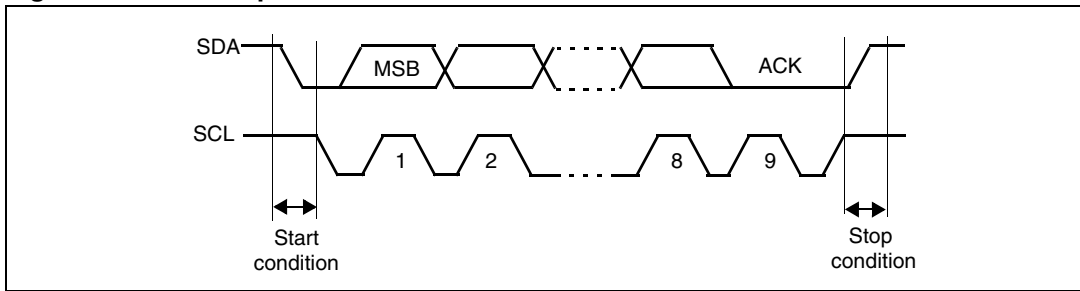
Figure 215. I 2 C bus protocol
