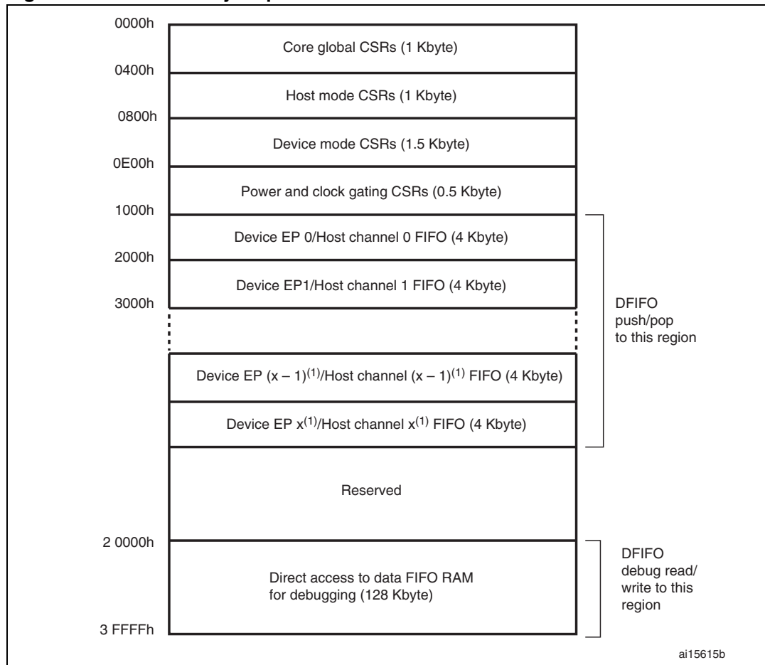
Figure 357. CSR memory map
