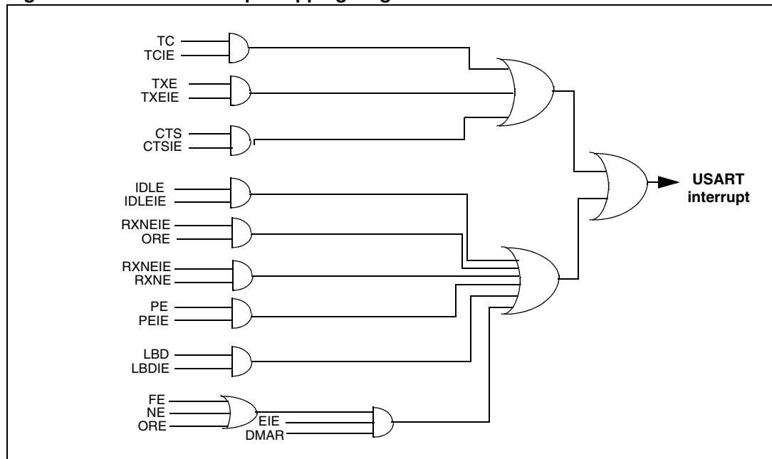
Figure 246. USART interrupt mapping diagram
