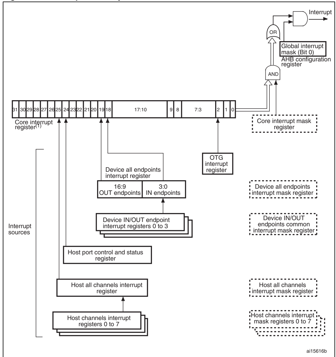
Figure 356. Interrupt hierarchy
