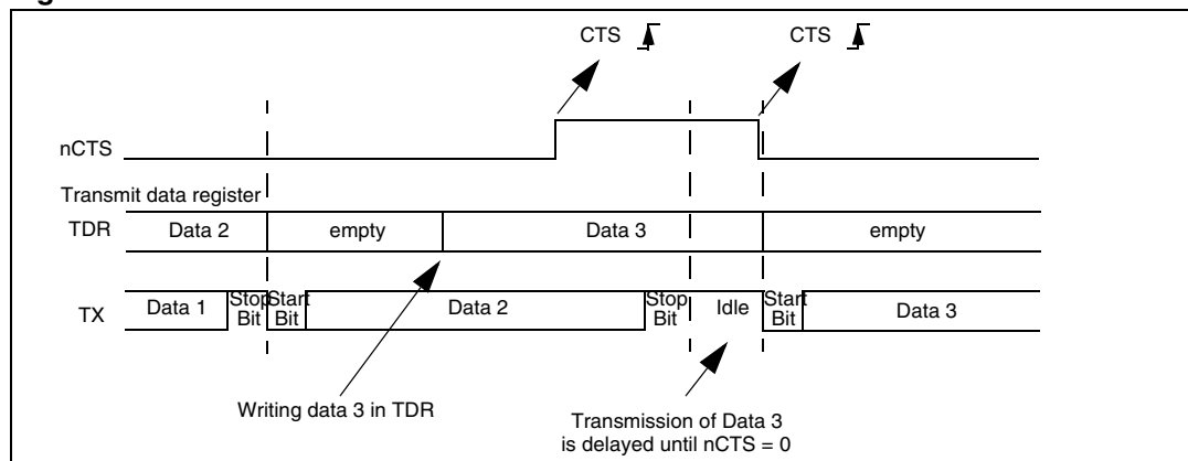
Figure 245. CTS flow control
