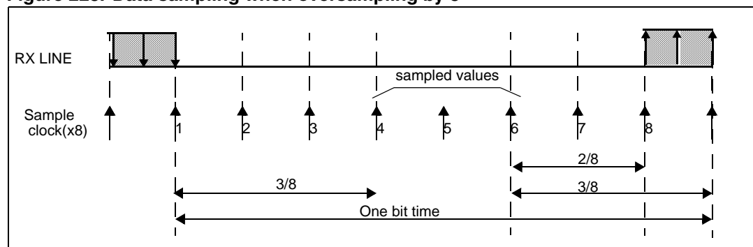
Figure 228. Data sampling when oversampling by 8
