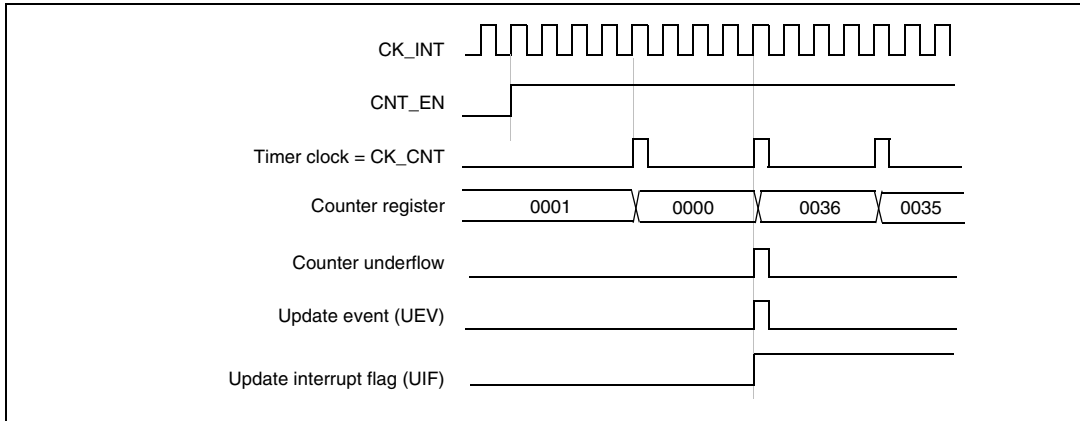
Figure 124. Counter timing diagram, internal clock divided by 4
