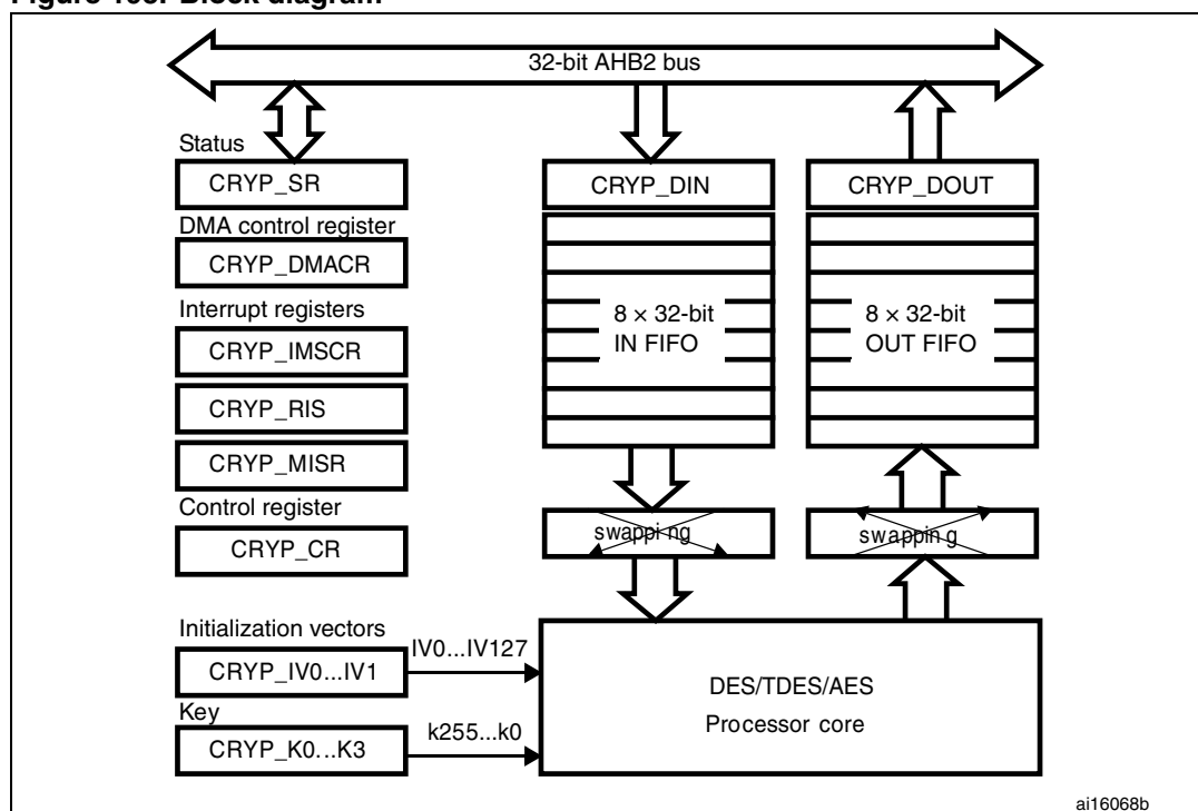
Figure 195. Block diagram
