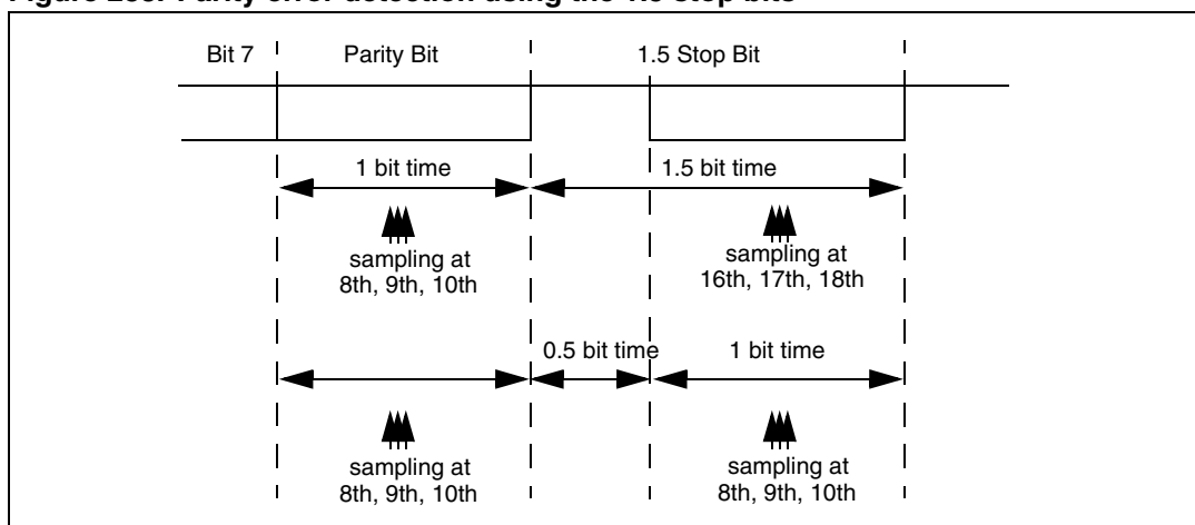
Figure 238. Parity error detection using the 1.5 stop bits
