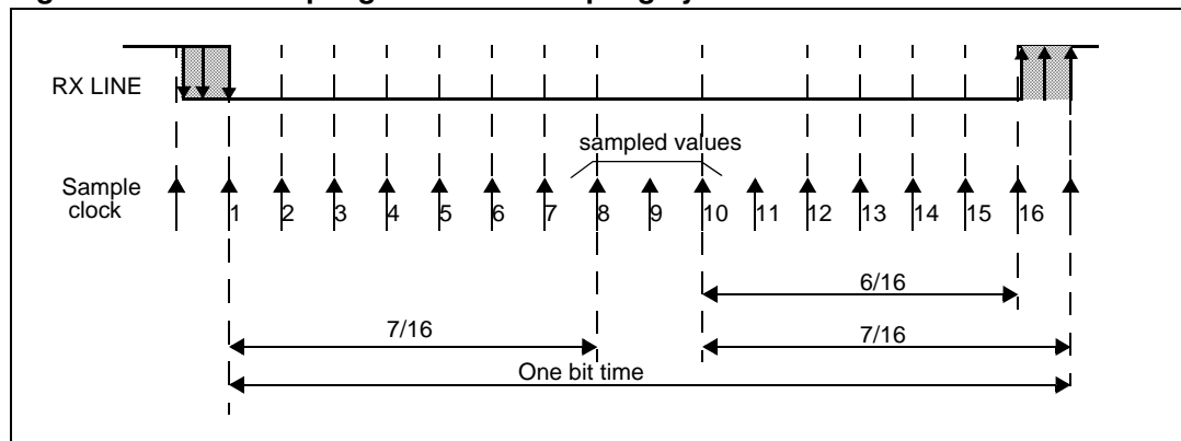
Figure 227. Data sampling when oversampling by 16
