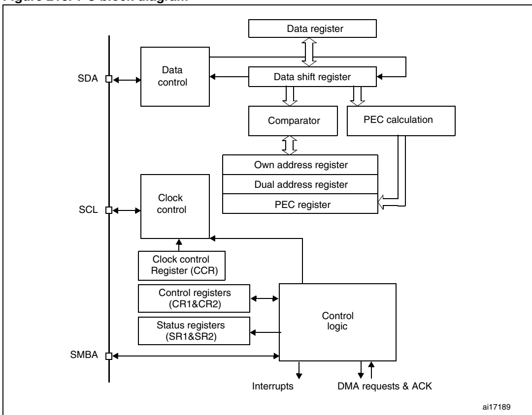
Figure 216. I 2 C block diagram
