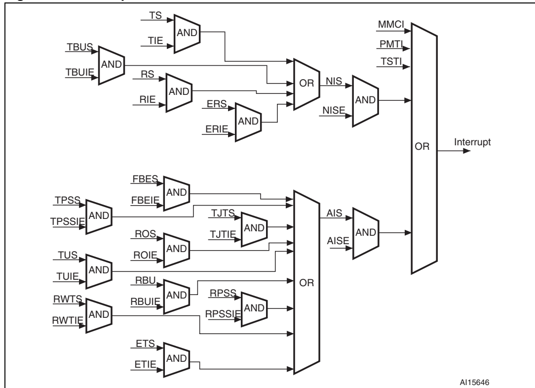
Figure 346. Interrupt scheme
