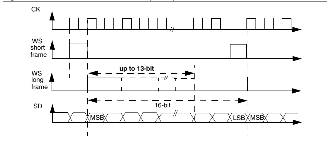
Figure 280. PCM standard waveforms (16-bit)
