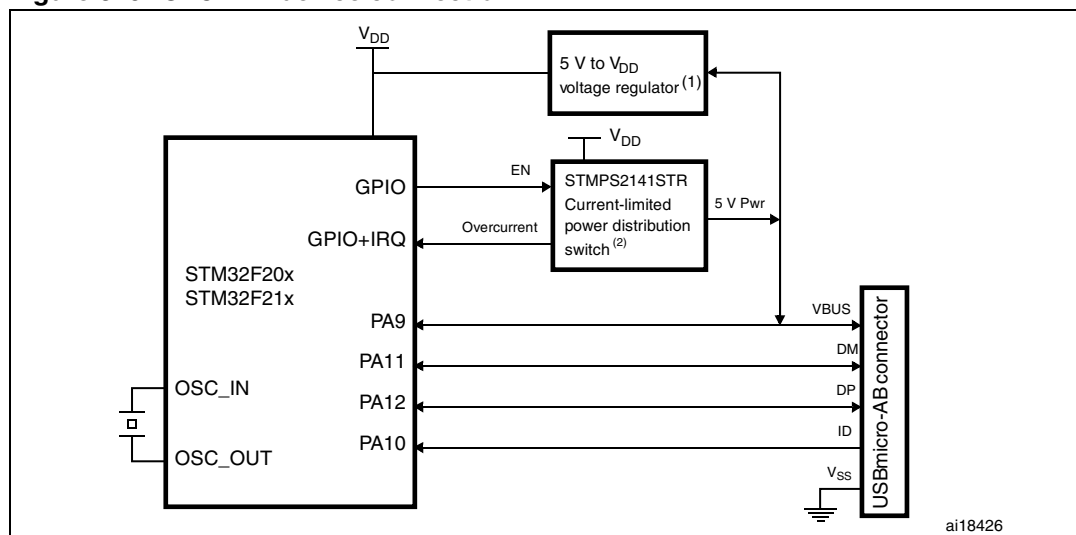
Figure 349. OTG A-B device connection
