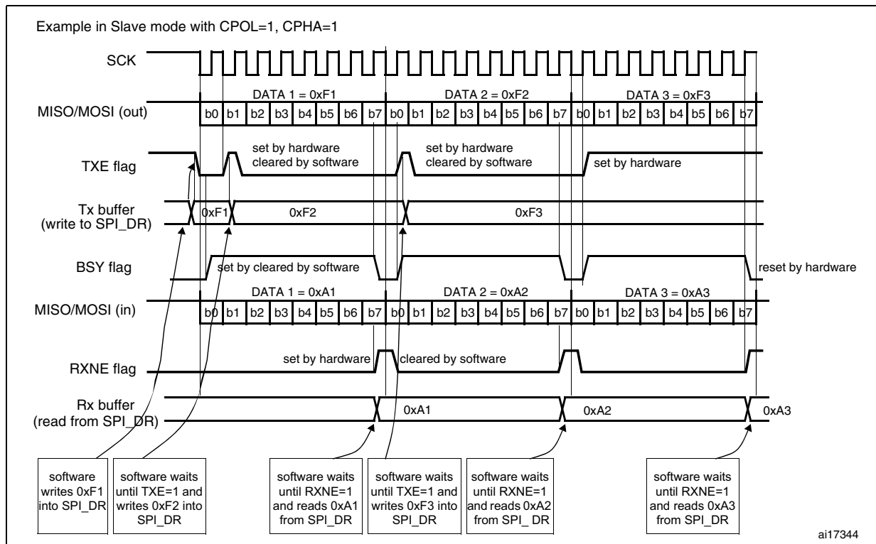
Figure 256. TXE/RXNE/BSY behavior in Slave / full-duplex mode (BIDIMODE=0, RXONLY=0) in the case of continuous transfers
