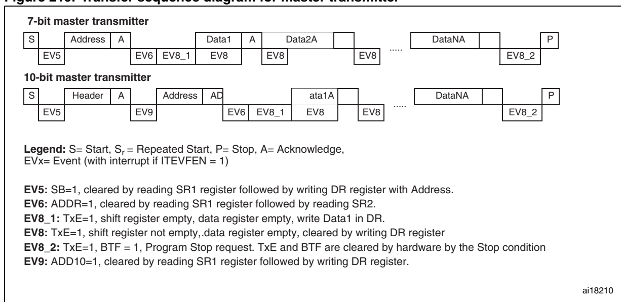
Figure 219. Transfer sequence diagram for master transmitter
