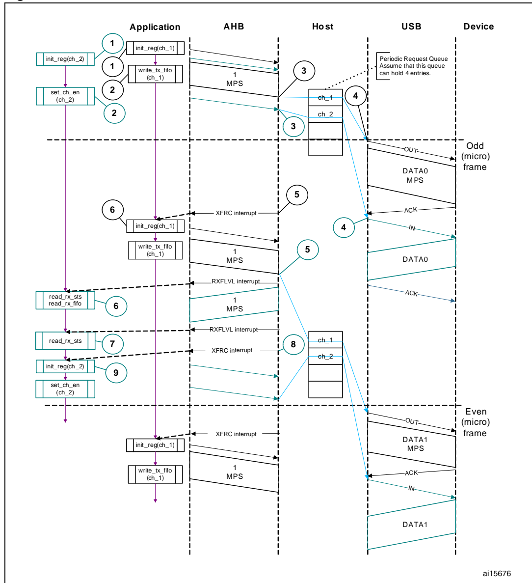
Figure 363. Normal isochronous OUT/IN transactions
