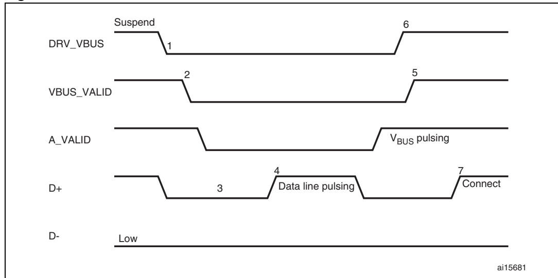
Figure 368. A-device SRP
