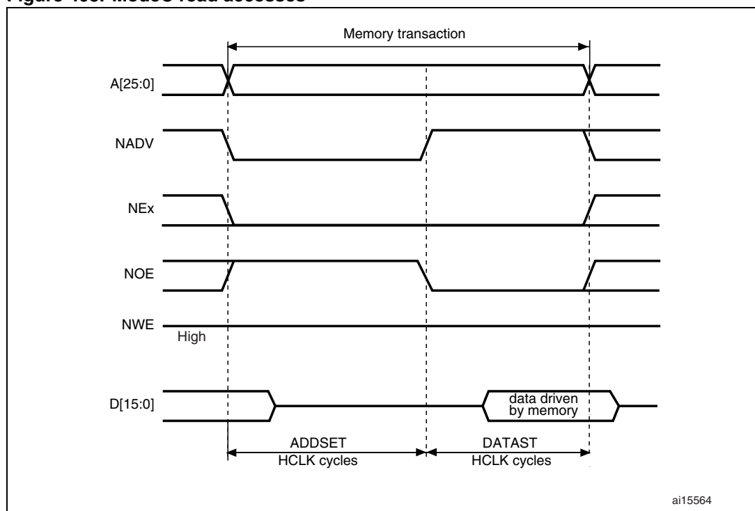
Figure 403. ModeC read accesses
