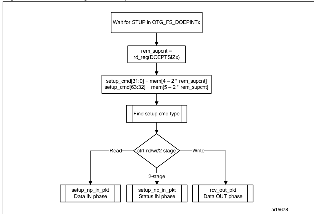
Figure 365. Processing a SETUP packet
