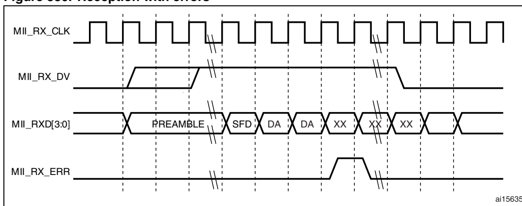
Figure 330. Reception with errors
