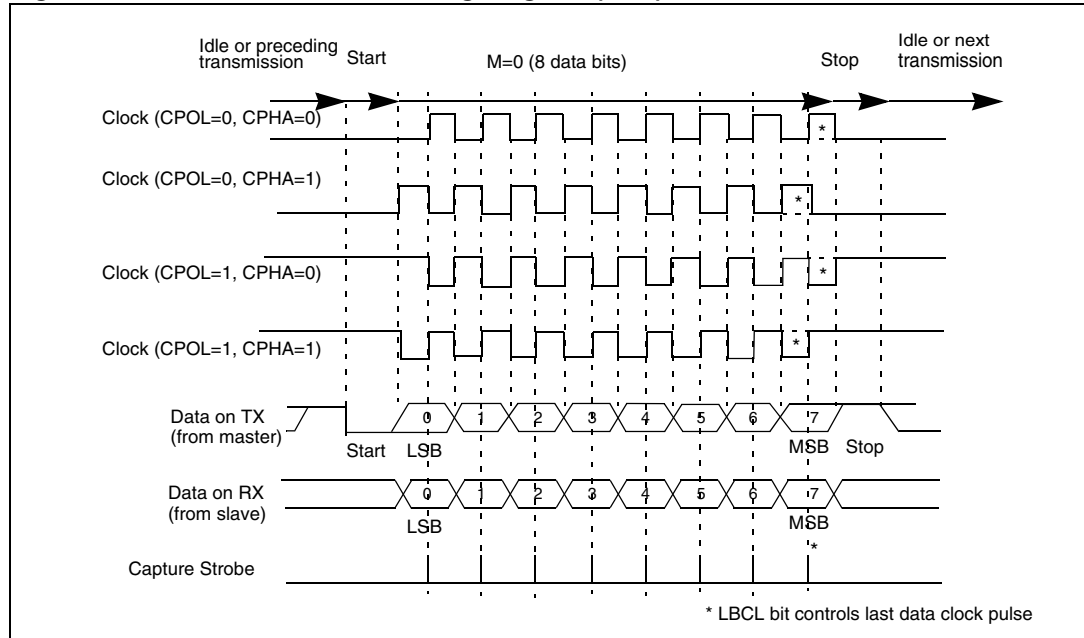
Figure 234. USART data clock timing diagram (M=0)
