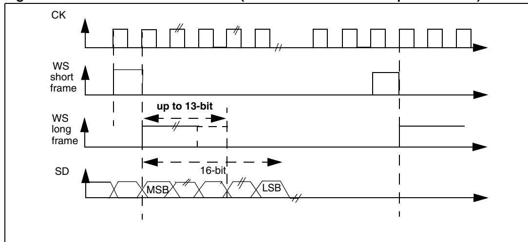
Figure 281. PCM standard waveforms (16-bit extended to 32-bit packet frame)
