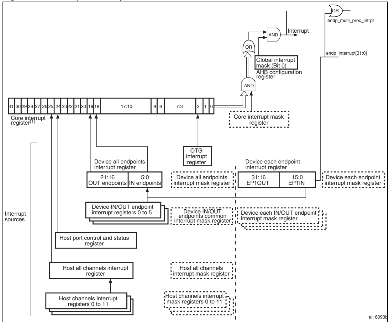
Figure 374. Interrupt hierarchy
