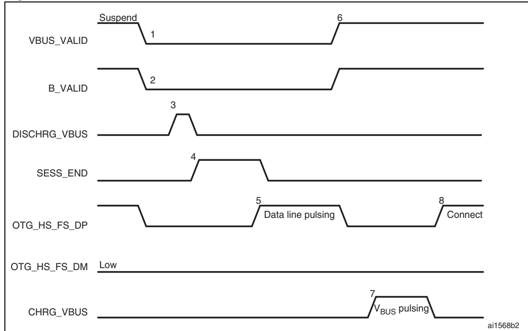
Figure 391. B-device SRP
