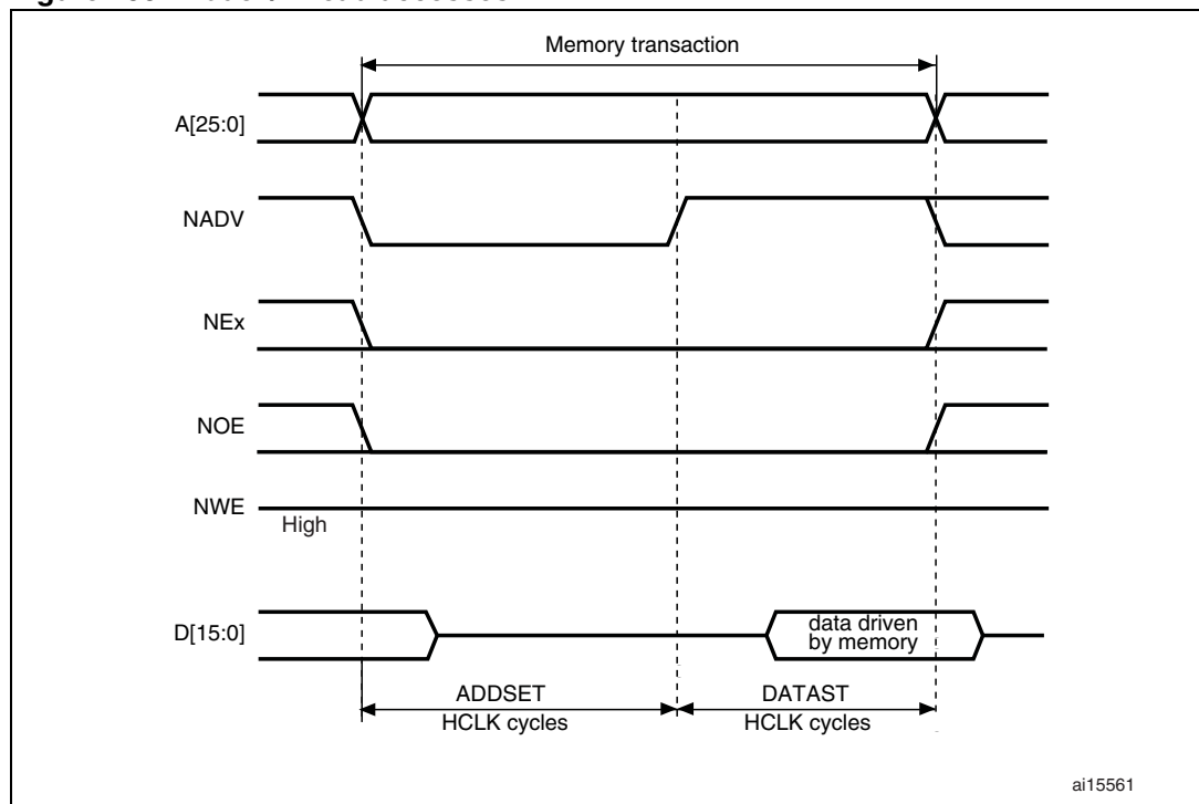
Figure 400. Mode2/B read accesses
