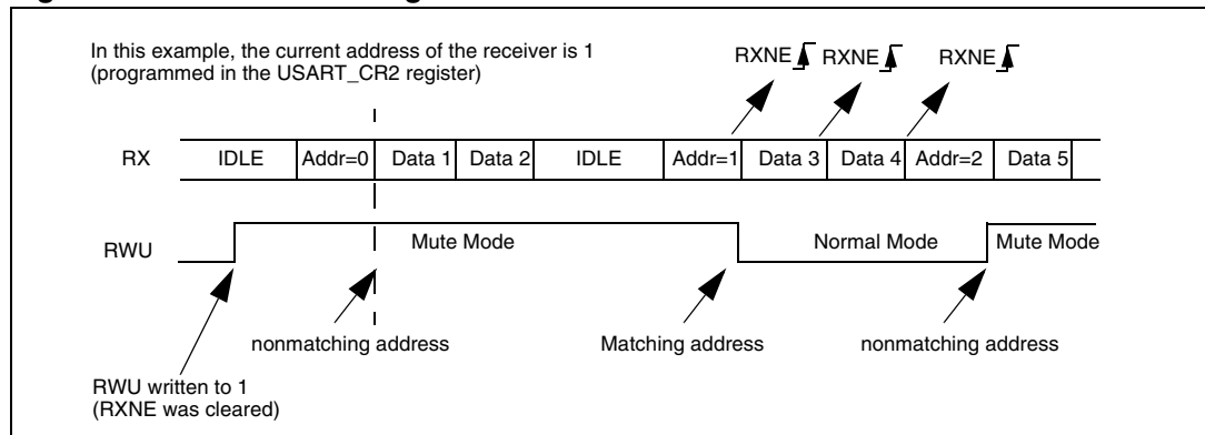
Figure 230. Mute mode using address mark detection
