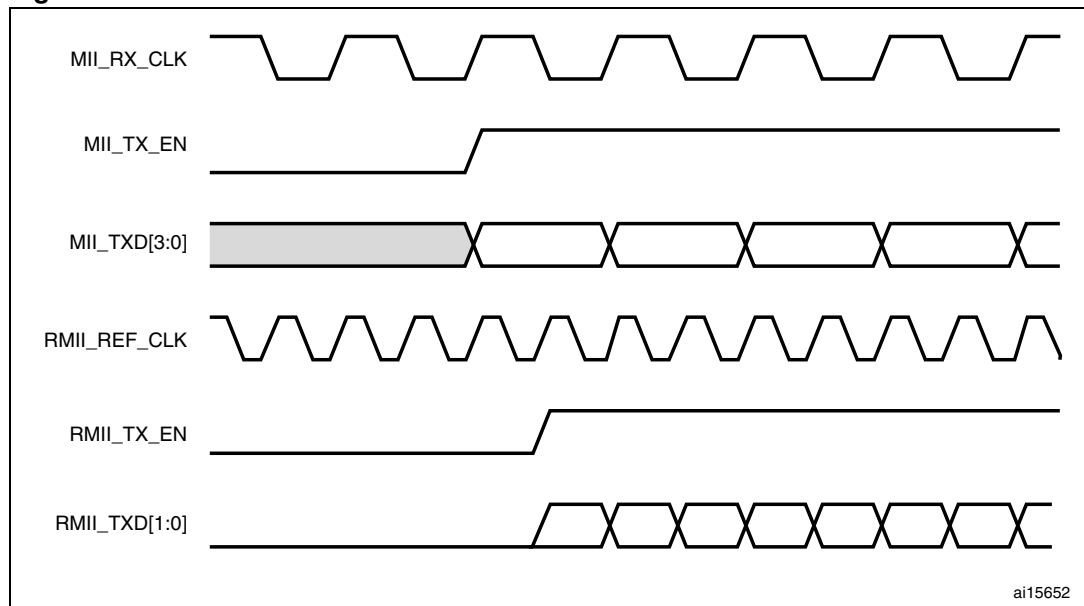
Figure 327. Frame transmission in MII and RMII modes
