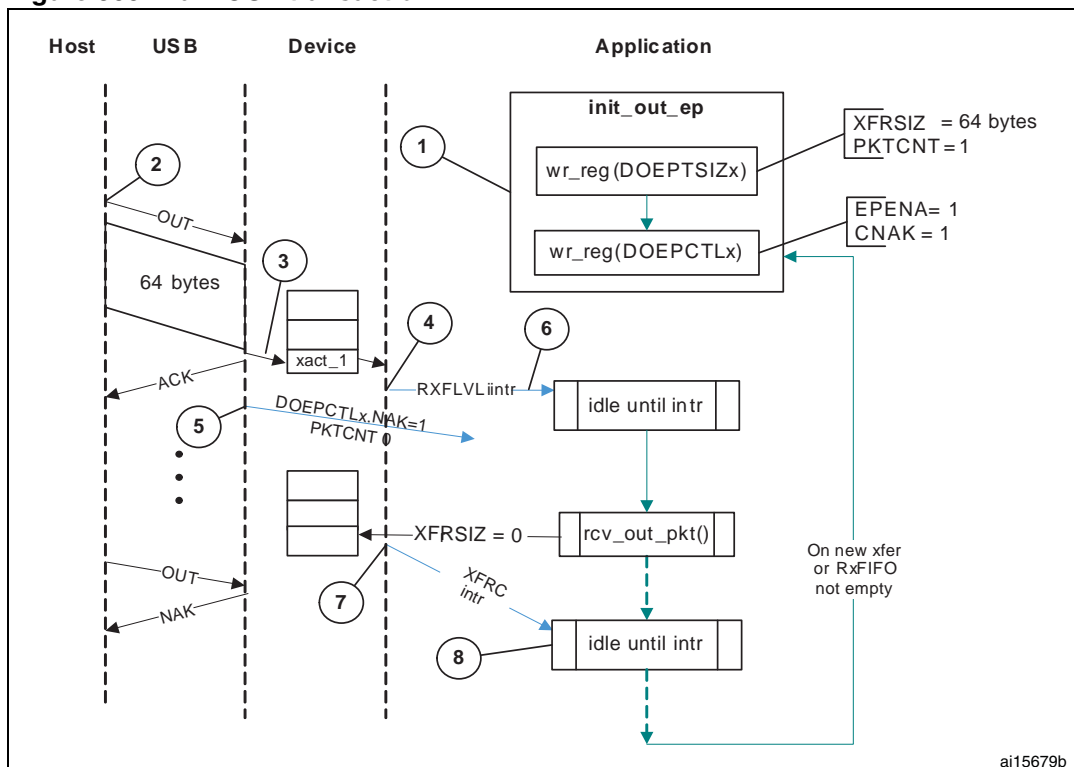
Figure 366. Bulk OUT transaction
