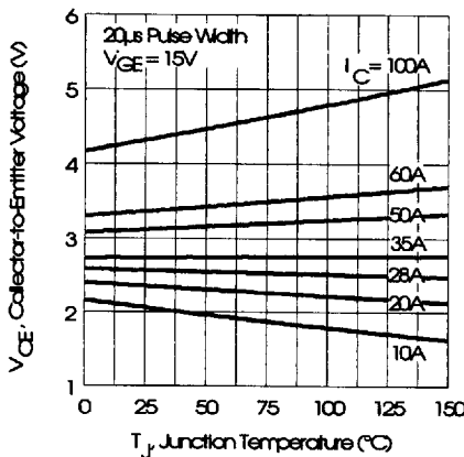
Fig. 5 - Collector-to-Emitter Saturation Typical Voltage vs. Junction Temperature
