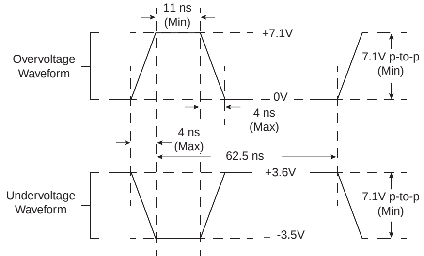
Figure 6. Maximum AC Waveforms for 3.3V Signaling
