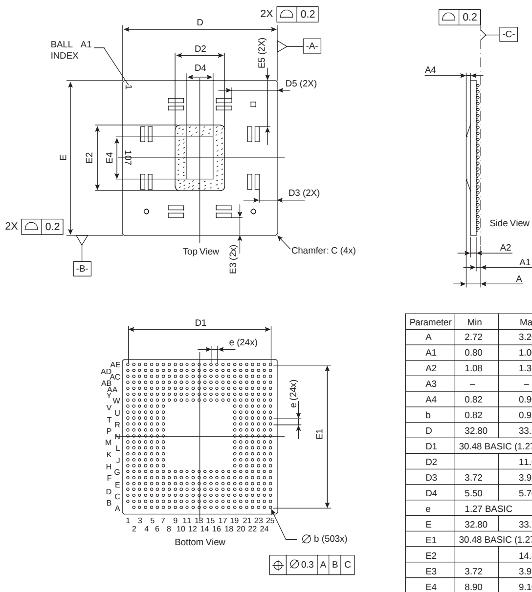
Figure 29. Mechanical Dimensions and Bottom Surface Nomenclature of the 503-ball HiTCE Package
