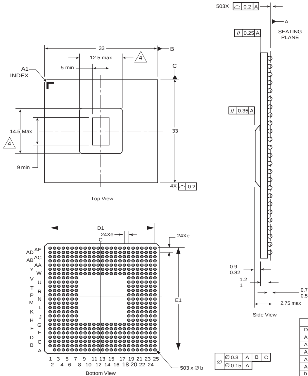
Figure 28. PC107A Package Dimensions and Pinout Assignments
