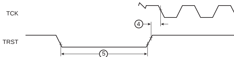
Figure 25. JTAG TRST Timing Diagram
