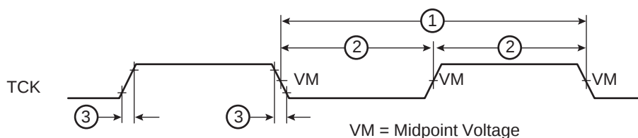
Figure 24. JTAG Clock Input Timing Diagram
