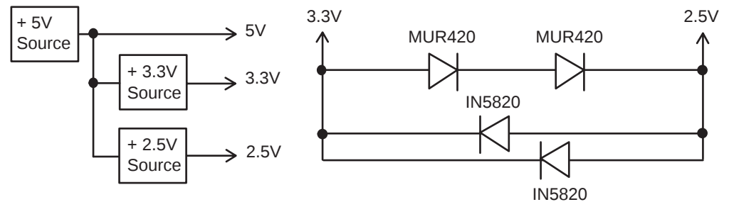
Figure 31. Example Voltage Sequencing Circuits
