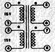
BASIC SCHEMATIC
