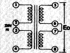
SERIES CONNECTED
